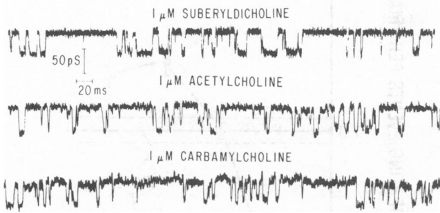
FIGURE 1 Single-AChR-channel currents activated by different cholinergic agonists. Planar lipid bilayers were formed in 0.5 M NaCl, 5 mM CaCl 2 , 2.5 mM HEPES, pH 7.4. SubCh (upper record), ACh (middle record) and CCh (lower record) were added to the cis-side of the membrane. V = -70 mV, negative in the compartment containing the agonist. The open channel conductance, \gamma = 48 pS for all three agonists.
