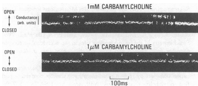
FIGURE 10 Frequency of channel opening in the presence of CCh. Monte Carlo simulations using the four-state model (Fig. 9) are displayed in the format of Fig. 6. Upper panel : 1 mM CCh. Lower panel : 1 \mu\text{M} CCh.
