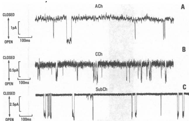
FIGURE 5 Single-channel currents activated by different cholinergic agonists and recorded in bilayers formed at the tip of patch pipets. ACh ( 10 \mu\text{M} ) (upper record): V = -51 mV. CCh ( 10 \mu\text{M} ) (middle record): V = -10 mV. SubCh, ( 10 nM) (lower record): V = -100 mV. The single-channel conductance \gamma = 40 \pm 5 pS for all three agonists. The seal resistances were 17 \text{ G}\Omega , 5 \text{ G}\Omega and 10 \text{ G}\Omega , respectively. The records were low-pass filtered at 1 KHz. Other conditions as for Fig. 1 (from Suarez-Isla et al., 1983).
