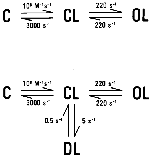
FIGURE 9 Models of AChR channel kinetics. Upper panel : A three-state model consisting of two closed states (unliganded [C] and liganded [CL]) and one open-liganded state [OL]. Lower panel : A four-state model including a functionally desensitized (liganded) state [DL]. The rates shown consider agonist binding to be diffusion-limited with a K_D of 30 \mu\text{M} . Channel opening and closing rates are measured results, and rates for desensitization and for recovery from desensitization are taken from Sakmann et al. (1980) channel data and Walker et al. (1982) flux measurements.
