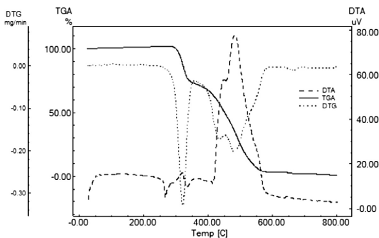
Figure 2 TGA, DTG and DTA curves of doxazosin mesilate.
