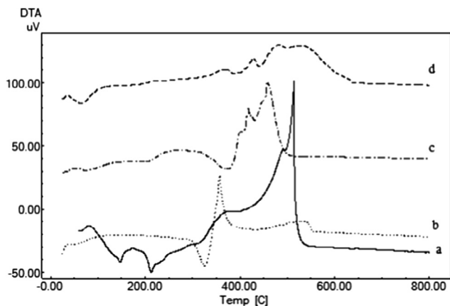
Figure 5 DTA curves of doxacor tablets (a), microcrystalline cellulose (b), magnesium stearate (c) and povidone (d).
