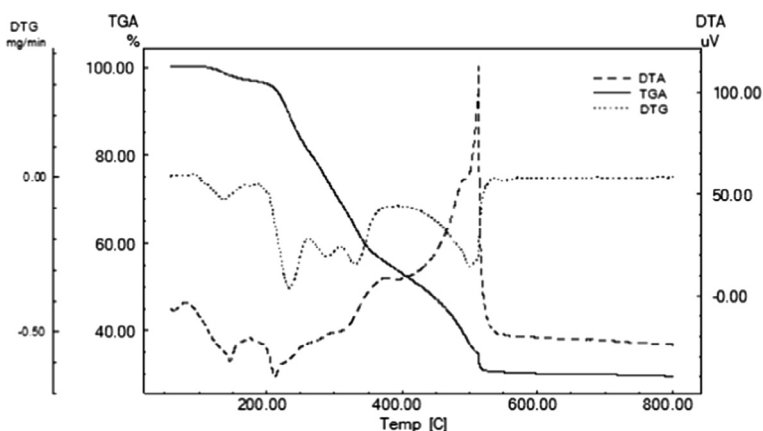
Figure 4 TGA, DTG and DTA curves of doxacor tablets.
