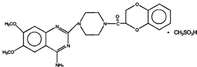
Figure 1 Chemical structure of doxazosin mesilate.
