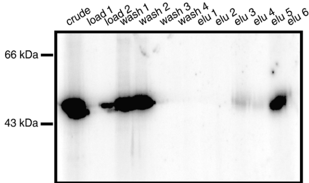
Fig. 2. Partial purification of the Ser274 protein kinase using peptide affinity chromatography. After the protein kinase was washed off the plasma membrane with 0.5 M KCl, the fraction was desalted. The kinase activity was purified on an affinity matrix with the peptide RAAAIKALGSFRSNPTN, corresponding to the phosphorylation site around Ser274, bound to the matrix. The fractions were: crude (desalted fraction), load 1 and 2 (not bound to the column, coming out when loading the column), wash 1 to 4 (not bound to the column, coming out when washing the column with buffer to remove unbound molecules), and elu 1 to 6 (bound to the column and eluted with 0.5 M NaCl). 4.8 \mu L fraction was loaded in each lane, corresponding to the protein amounts 5.77 \mu g crude, 0 \mu g load 1, 0.10 \mu g load 2, 0.69 \mu g wash 1, 0.34 \mu g wash 2, 0 ng each of wash 3, wash 4 and elu 1, 4.93 \mu g elu 2, 5.15 \mu g elu 3, 0.91 \mu g elu 4, 1.16 \mu g elu 5 and 1.41 \mu g elu 6. The kinase activity was eluted in fraction 5. The kinase activities in the different fractions were detected by in vitro phosphorylation assays. The fractions were incubated with MBP-Ser274 and [ \gamma - 32 P]-ATP in the phosphorylation buffer for 30 min at room temperature, whereafter the reaction mixtures were separated by SDS-PAGE and the radiolabelled polypeptides visualized using a PhosphorImager.
