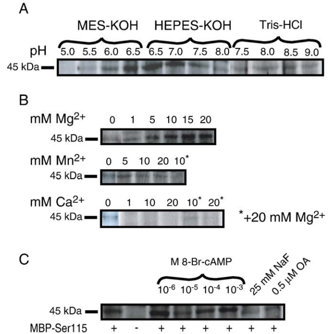
Fig. 3. Characterization of the Ser115 protein kinase. The different conditions were tested using in vitro phosphorylation assays, in which the kinase fractions were incubated with MBP-Ser115 and [ \gamma - 32 P]-ATP in the phosphorylation buffer for 30 min at room temperature. The reaction mixtures were separated by SDS-PAGE and the radio labelled polypeptides were visualized using a PhosphorImager. Additional weaker bands were also detected on the gels (not shown in the figure), which probably arise from other proteins in the fraction that are phosphorylated and/or autophosphorylated. (A) The protein kinase had a pH optimum at 6.5. (B) The kinase required Mg 2+ for activity, and was inhibited by mM concentrations of Mn 2+ and Ca 2+ . (C) The phosphorylation was not increased by the cyclic AMP-analogue 8-Br-cAMP, or the phosphatase inhibitors sodium fluoride (NaF) and okadaic acid (OA).
