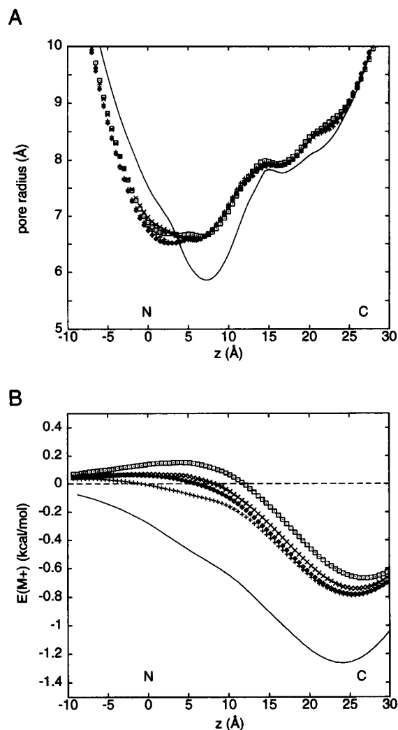
FIGURE 9 Comparison of the \alpha 7 and Torpedo open conformation models. (A) The pore radius profiles of \alpha 7 (solid line) and of four Torpedo ( \diamond , \beta a ; + , \beta c ; \square , \gamma a ; \times , \gamma c ) models are compared. (B) The electrostatic potential energy profiles for the same four Torpedo ( \diamond , \beta a ; + , \beta c ; \square , \gamma a ; \times , \gamma c ) models are given.
