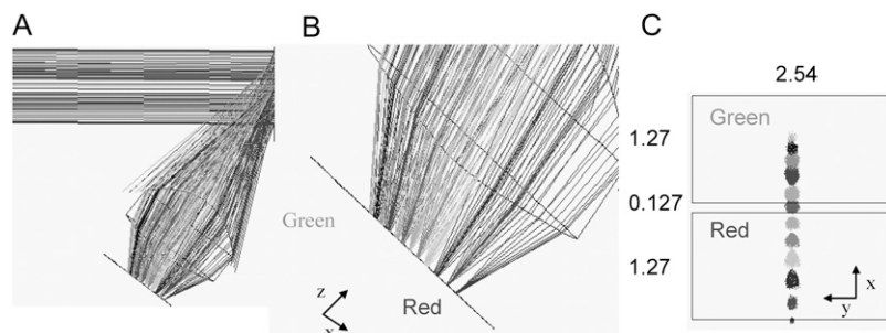
FIGURE 6 (A) ZEMAX simulation using 12 sample wavelengths. The central wavelength is 655 nm. (B) Zoom in of the yz image plane. (C) Image on the xy image plane with grid representing the photodiode surface. Units are in millimeters.
