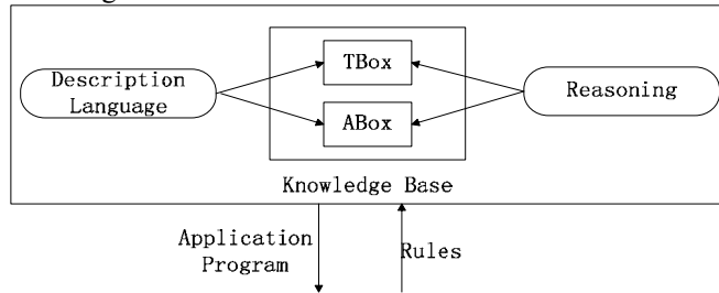
Fig.1 Description Logic-based knowledge representation System
