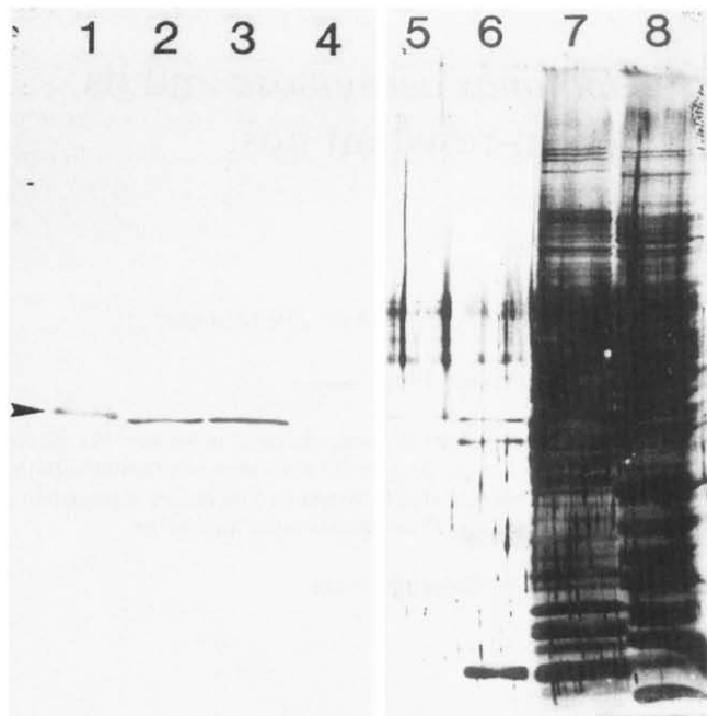
Fig. 1. Western blotting analysis of D2. Samples were subjected to SDS-polyacrylamide gel (10%) electrophoresis. Protein was blotted to polyvinylidene difluoride membrane (Millipore) at 300 mA for 30 min. Lanes 1 through 4 were stained with the anti-D2 IgG. Lanes 5 through 8 were visualized with gold stain. Lane 1 and 5, purified D2 (70 ng); lane 2 and 6, strain PAO1 outer membrane (1 \mu g protein); lane 3 and 7, whole cell lysate of strain PAO1 (10 \mu g protein); lane 4 and 8, whole cell lysate of E. coli XL1-BLUE (10 \mu g protein). An arrowhead represents protein D2.
