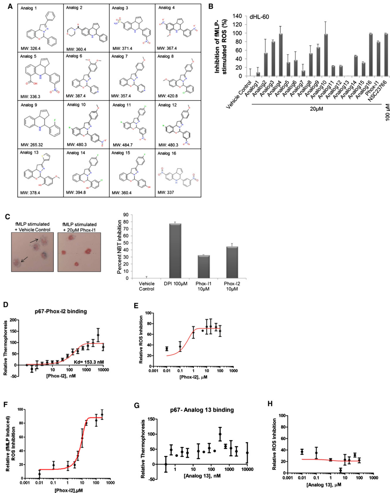
Figure 4. Phox-11-Analog Analysis Yields Compounds with Improved or Similar Cellular ROS Inhibitory Activity
