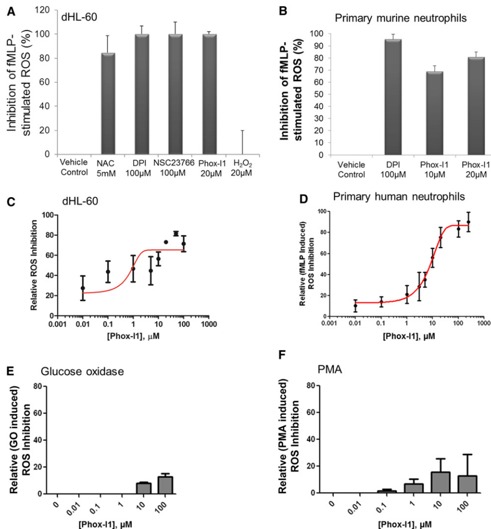
Figure 3. fMLP-Stimulated ROS Production Is Abrogated by Phox-11 in Human HL-60 Cells and Primary Murine Neutrophils
