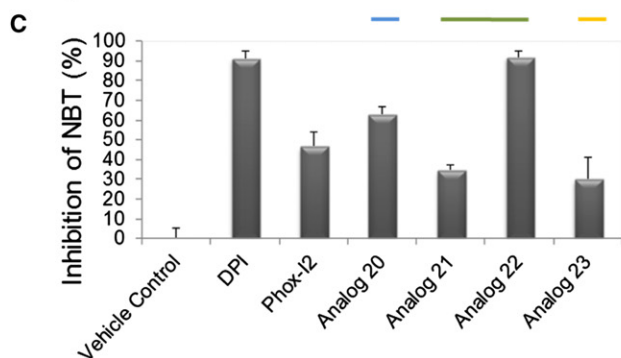
Figure 6. Medicinal Chemistry Optimization of Phox-I2 Allows for the Replacement of Potentially Toxic Nitro Groups
