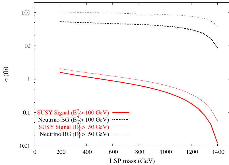
Fig. 3. Cross sections of the higgsino signal (14) and neutrino background (15) at CLIC with polarized e^- and e^+ beams. Initial state radiation is included.
