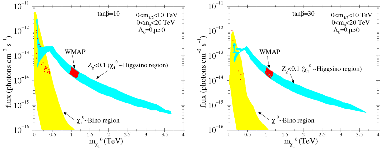
Fig. 5. Monochromatic gamma ray flux from DM pair annihilation near the galactic center shown for the NFW profile of DM halo distribution and an aperture \Delta\Omega = 10^{-3} sr.
