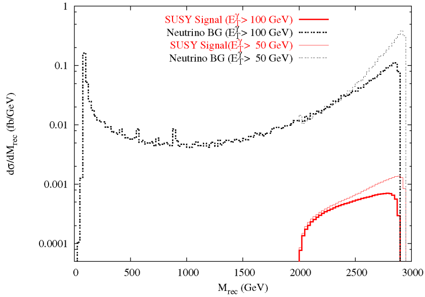
Fig. 4. The recoil mass distributions of a 1 TeV higgsino signal (14) and the neutrino background (15) at CLIC with polarized e^- and e^+ beams. Initial state radiation is included.
