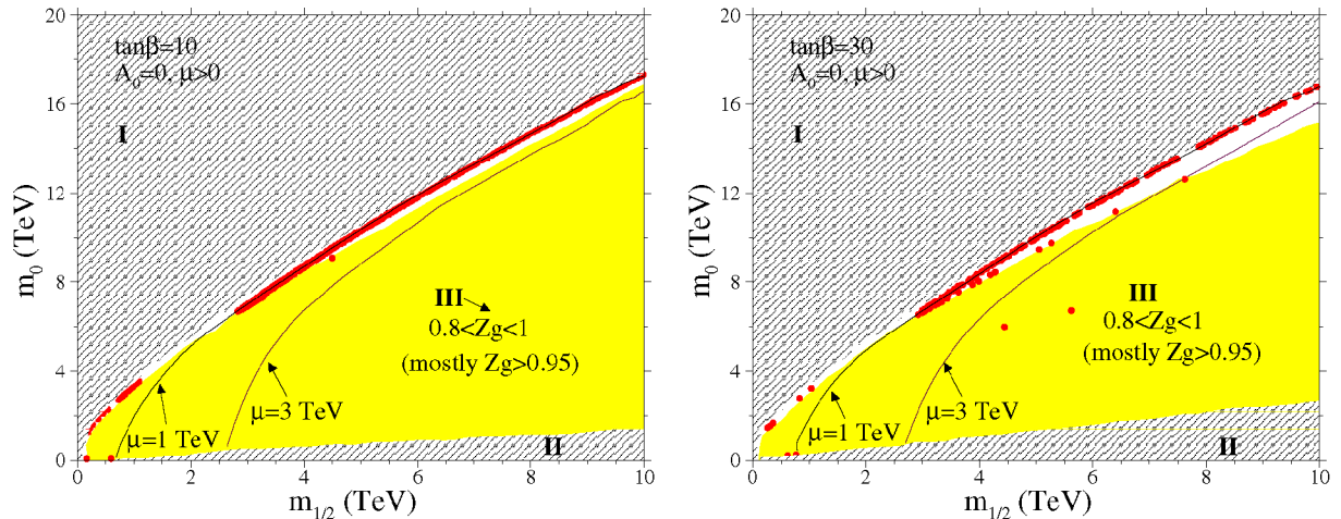
Fig. 1. mSUGRA parameter space for m_t = 178 GeV, A_0 = 0 and \tan\beta = 10 (left) and 30 (right). The patterned regions marked I and II are disallowed by the EWSB condition and the constraint of a neutral LSP, respectively. In the large grey (yellow in web version) region the LSP is bino-like. Points (red in web version) satisfy the constraint (8) on the dark matter relic density.
