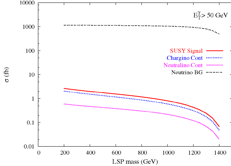
Fig. 2. Cross sections for the higgsino signal (14) and the neutrino background (15) at CLIC ( \sqrt{s} = 3 ) TeV, produced with a photon tag of E_T^\gamma > 50 GeV. Initial state radiation is included.
