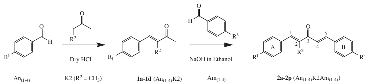
Scheme 1. Reaction conditions for the synthesis of the assayed compounds, using p -substituted aldehydes A1 ( R^1, R^3 = H ), A2 ( R^1, R^3 = OCH_3 ), A3 ( R^1, R^3 = NO_2 ) and A4 ( R^1, R^3 = N(CH_3)_2 ) and butanone (K2, R^2 = CH_3 ) resulting in 1a–1d , respectively; and further reaction of each enone 1a–1d with same aldehydes to give the collection An_{(1-4)}K2Am_{(1-4)} ( 2a–2p ).
