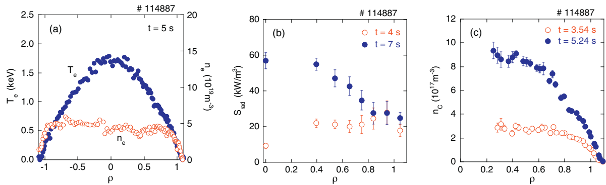
Fig. 2. Radial profiles of (a) electron temperature and density, (b) radiated power density and (c) carbon density along normalized minor radius \rho in the long pulse discharge (#114887).
