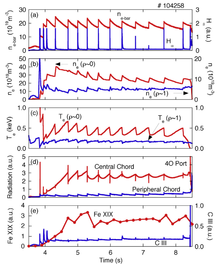
Fig. 4. Long pulse operation with super dense core (SDC) plasma by multiple pellet injection in the magnetic configuration R=3.75 \text{ m} . Time evolutions of (a) averaged electron density and H_{\alpha} signal, (b) central and edge electron densities, (c) central and edge electron temperature, (d) line-integrated radiation in the central and peripheral chord, (e) impurity line intensities of Fe XIX and C III are indicated.
