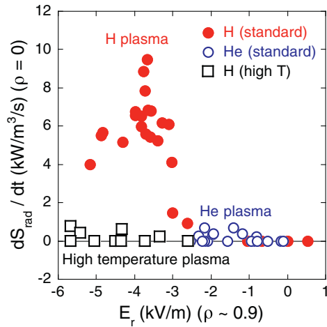
Fig. 11. Relationship between the radial electric field at the plasma edge and the increasing rate of core radiation in standard H, He and high temperature plasmas.
