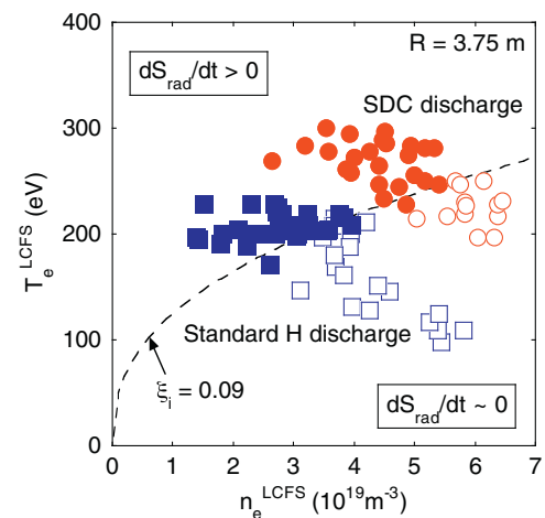
Fig. 8. Mapping of SDC plasmas and standard hydrogen plasmas on n - T space at the plasma edge. Both SDC and standard hydrogen plasmas are produced in the magnetic configuration R=3.75 m. The closed and open symbols indicate the plasmas with and without impurity accumulation at each time in the discharges (e.g. # 104258 in Fig. 4), respectively. The dashed line is fitted by the curve of constant \xi_i parameter.
