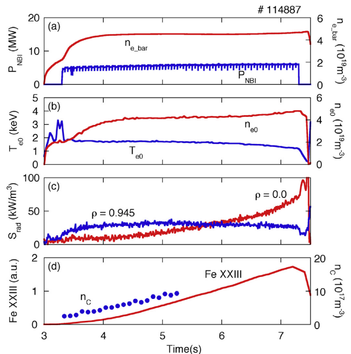
Fig. 1. Typical long pulse discharge with impurity accumulation. Time evolutions of (a) heating power of neutral beam injection and averaged electron density, (b) central electron temperature and density, (c) radiated power densities in the center and the peripheral region, (d) impurity line intensity and central carbon density are indicated.
