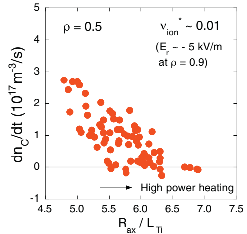
Fig. 12. Correlation between the increasing rate of carbon density and ion temperature gradient in hydrogen plasmas with the constant ion collisionality ( \nu_{\text{ion}}^* \sim 0.01 ) at \rho = 0.5 . The ion collisionality corresponds to that of 0.025 at \rho = 1.0 and E_r \sim -5 kV/m at the plasma edge ( \rho \sim 0.9 ).
