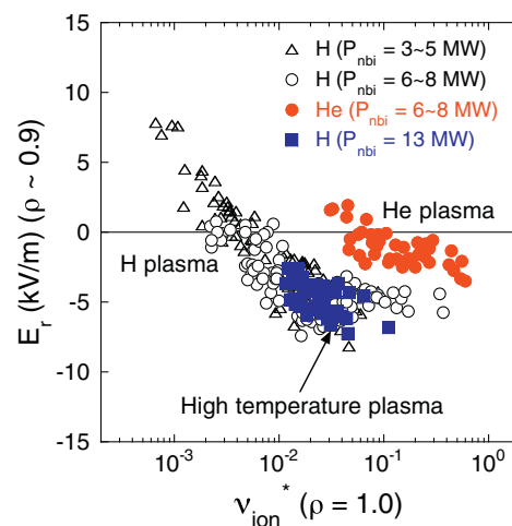
Fig. 10. Radial electric field in the plasma edge region as a function of background ion collisionality for H and He plasmas with different heating powers.
