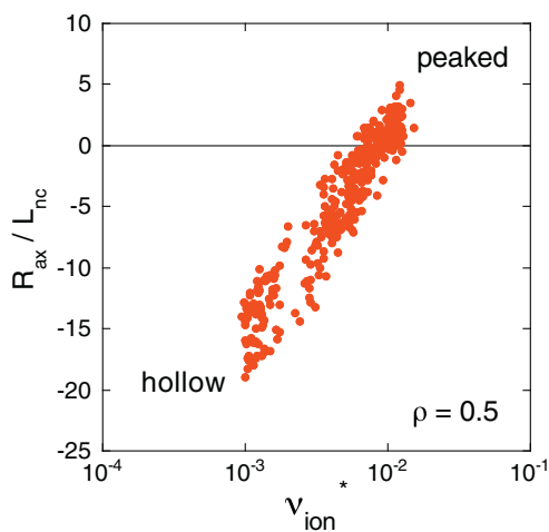
Fig. 14. Correlation between carbon density profile and ion collisionality. The vertical axis indicates the normalized logarithmic carbon density gradient ( R_{ax}/L_{nc} ) at the mid-radius.
