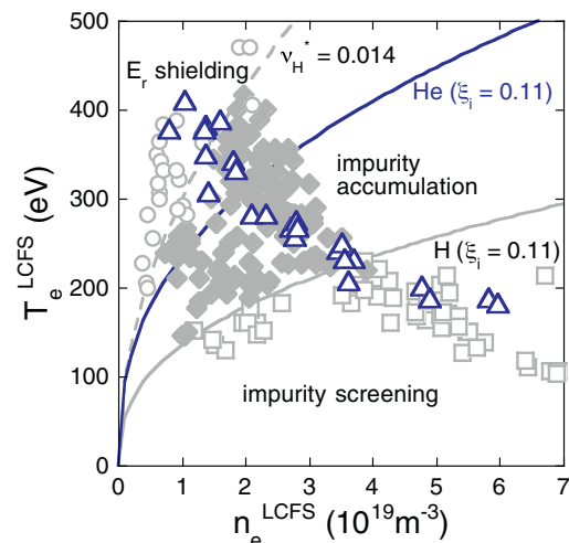
Fig. 9. Mapping of He rich plasmas and standard hydrogen plasmas on n - T space at the plasma edge. The light gray symbols and open triangles indicate hydrogen plasmas and He rich plasmas, respectively. The solid and dashed lines of light gray indicate the empirical scaling on impurity screening for hydrogen plasmas [21]. The bold solid line is estimated for pure helium plasmas by using the same \xi_i parameter for hydrogen plasmas.
