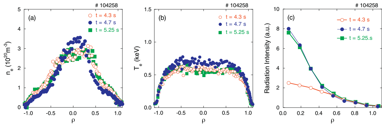
Fig. 5. Radial profiles of (a) electron density, (b) electron temperature and (c) local radiation intensity in the long pulse SDC discharge (#104258).
