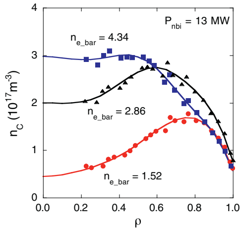
Fig. 13. Carbon density profiles in high temperature plasmas with different average densities. Each carbon density profile is maintained during the discharge.
