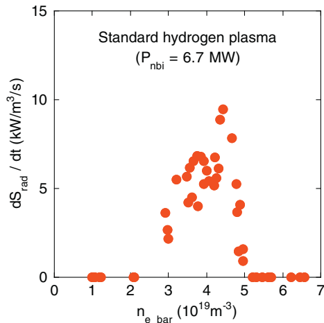
Fig. 3. Impurity accumulation window in density scan experiment with standard hydrogen plasmas. The observable indicator for impurity accumulation is the estimated increasing rate of central radiation.
