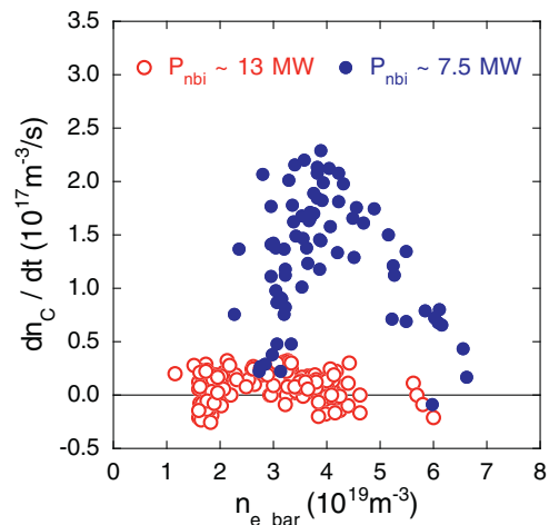
Fig. 7. Dependence of the increasing rate of core carbon density on averaged electron density for two different heating power cases ( P_{\text{nbi}} = 7.5 \text{ MW} and 13 \text{ MW} ).
