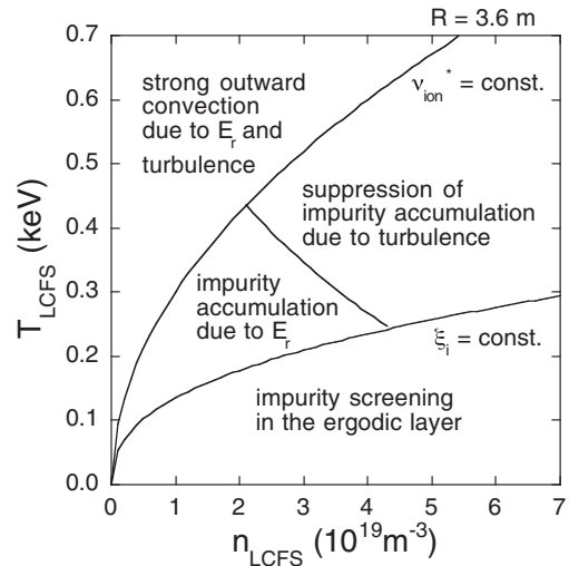
Fig. 15. Classification of impurity behavior on n - T space at the plasma edge in the operational regime on LHD with R=3.6 m. The n - T diagram is made for standard hydrogen plasmas with flat density and peaked temperature profiles. The dominant contribution to impurity transport is indicated in each domain. The solid lines are based on the empirical scaling determined by the mapping of various discharges.
