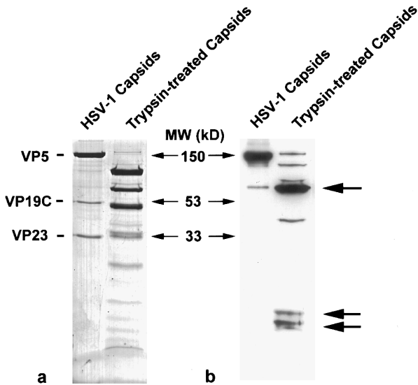
FIG. 2. SDS-PAGE and immunoblot analysis of full-length VP5 and tryptic fragments of VP5. The protein components of purified G-capsids (5 \mu g total protein) or trypsin-treated G-capsids (10 \mu g total protein) were separated on a 12% SDS-polyacrylamide gel. Proteins were visualized by Coomassie staining (a). A duplicate, unstained gel was electrophoretically transferred to an Immobilon membrane, and the blot was probed with mAb 6F10 (b). The large arrows on the right indicate proteolytic fragments that were further analyzed by protein sequencing.
