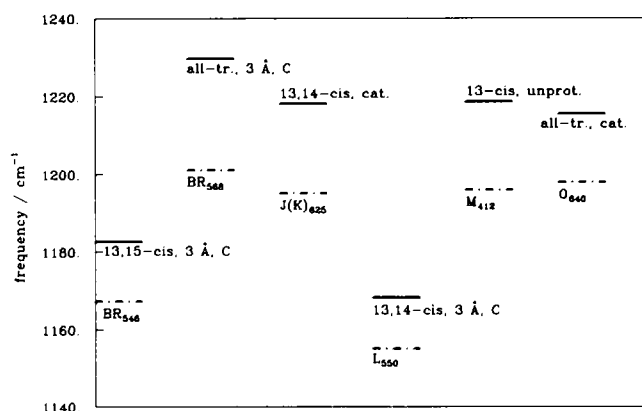
FIGURE 5 Comparison of calculated and observed \text{C}_{14}\text{-C}_{15} stretch frequencies for the 13,14- cis model shown in Fig. 4. The experimental assignments for \text{K}_{625} are from Gerwert et al. (20), those for \text{O}_{640} are from Smith et al. (12) and for \text{M}_{412} is our assignment according to a spectrum by Smith et al. (1). For the remaining assignments see the caption to Fig. 3.
