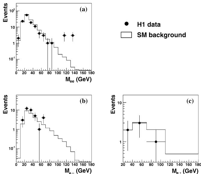
Fig. 2. Distribution of (a) the invariant mass M_{ee} of the two highest P_T electrons for multi-electron events, (b) the electron–muon invariant mass M_{e\mu} , and (c) the electron–tau candidate invariant mass M_{e\tau} . The data (symbols) are compared with the Standard Model expectation (histogram). The distributions are shown at the preselection level (see text).
