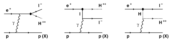
Fig. 1. Diagrams for the single production of a doubly-charged Higgs boson in e^+p collisions at HERA via the h_{e\ell} coupling. The hadronic final state is denoted by p(X) in the elastic (inelastic) case, where the initial proton remains intact (dissociates). The contribution of Z exchange can be safely neglected.
