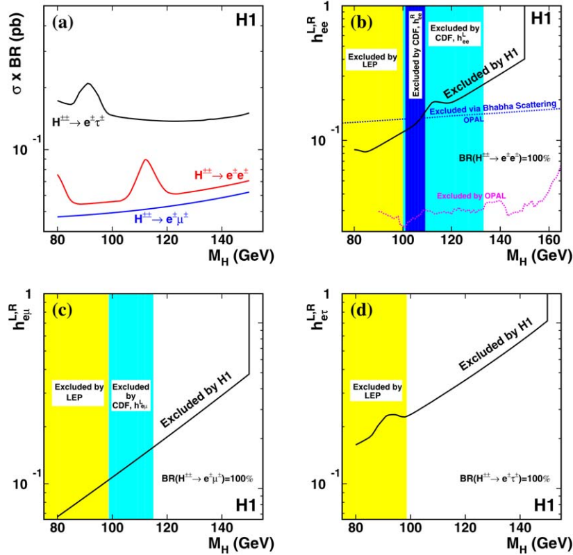
Fig. 3. (a) Upper limits at the 95% confidence level on the H^{\pm\pm} production cross section times the branching ratio for the H^{\pm\pm} to decay into ee , e\mu or e\tau , as a function of the Higgs mass. (b)–(d) Upper limits on the coupling h_{el} assuming that the H^{\pm\pm} couples only (b) to ee , (c) to e\mu or (d) to e\tau . Regions above the curves are excluded. The constraints obtained from pair production at LEP and at CDF and from single production at OPAL are also shown.
