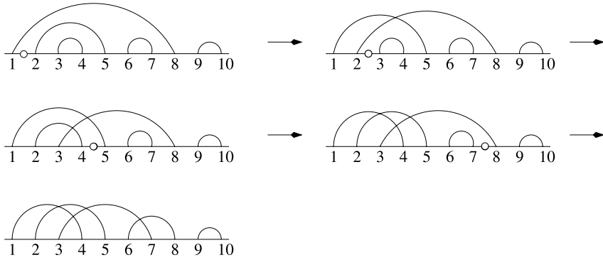
Fig. 4. Deleting neighbour nestings from an involution.
