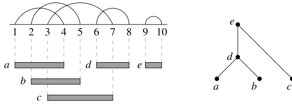
Fig. 2. The involution \pi = 45712836109 \in \mathcal{I}_{10} , the corresponding collection of intervals and the associated (2+2) -free poset.
