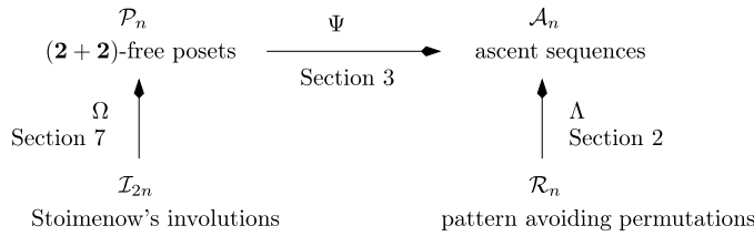
Fig. 1. The bijections of the paper.
