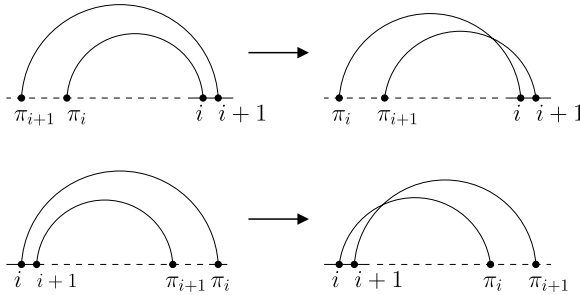
Fig. 3. Two operations on chord diagrams.
