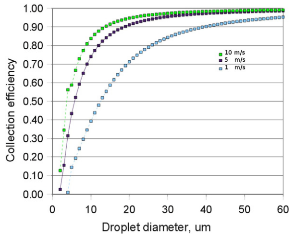
Fig. 2. Collection efficiencies for 1, 5 and 10 m s -1 relative wind speed and 0.6 mm wire diameter.
