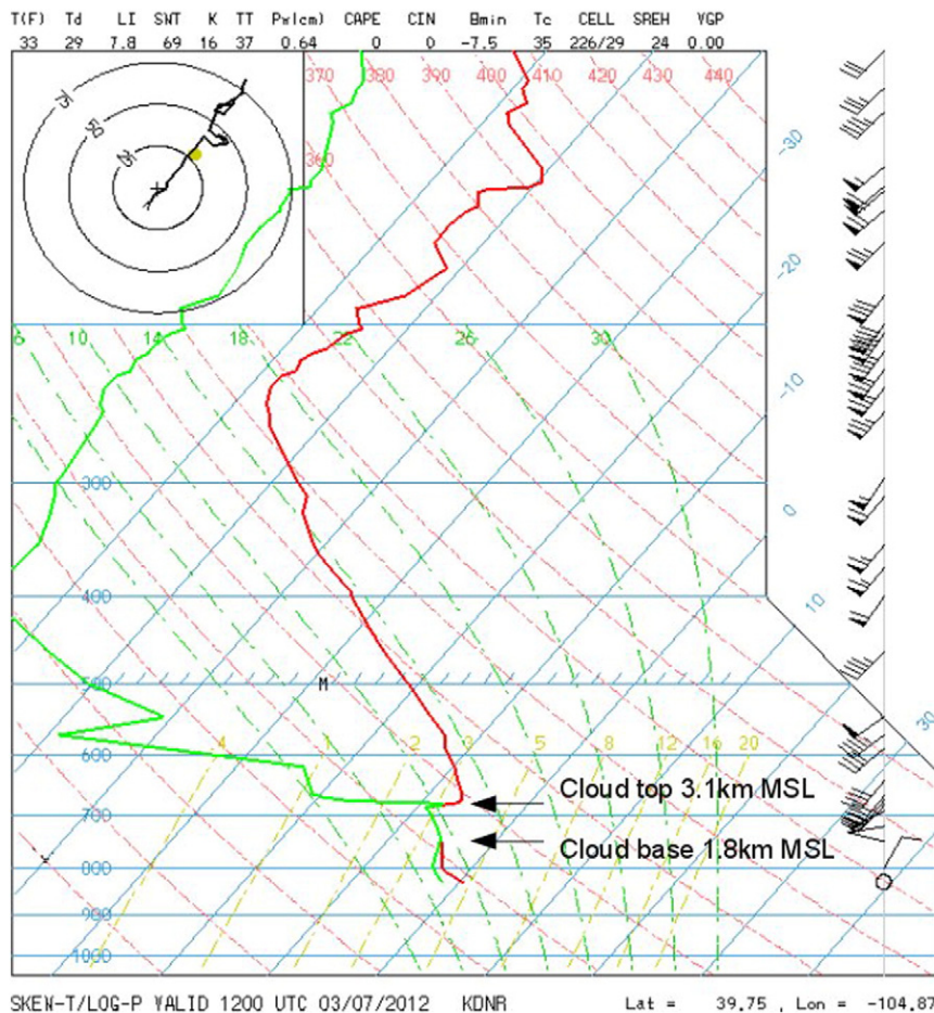
Fig. 3. Skew-T plot of temperature (red) and dewpoint temperature (green) from the National Weather Service radiosonde launched from Denver at 12 Z on March 7th, 2012.
