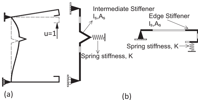
Fig. 4. Distortional buckling mode of a channel section with intermediate and edge stiffeners (a) distortional buckled shape and (b) equivalent struts.
