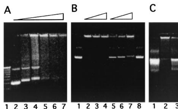
FIGURE 8 Agarose gel electrophoresis and EtBr staining of pCILuc cross-linked in C_{12}E_4 /TMP reverse micelles with W_o = 6.58 . (A) Lane 1, \lambda ladder; lane 2, unmodified DNA; lane 3, 1:0.02 labeled DNA; lane 4, 1:0.05 labeled DNA; lane 5, 1:0.1 labeled pCILuc; lane 6, 1:0.15 labeled DNA; lane 7, 1:0.2 labeled pCILuc. (B) Lanes 1–4, DNA oxidized in micelles; lanes 5–7, oxidized in water buffer; lane 1, unmodified DNA; lanes 2 and 5, DNA modified at 1:0.2 ratio; lanes 3 and 6, DNA modified at 1:0.5 ratio; and lanes 4 and 7, DNA modified at 1:1 ratio. (C) Lane 1, unlabeled control plasmid; lane 2, thiol DNA after micelle formation/oxidation; lane 3, thiol DNA after micelle formation/oxidation and reduction by 20 mM TCEP treatment 1 hr at 4°C.
