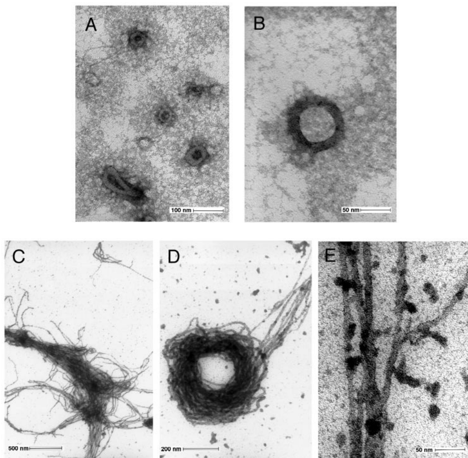
FIGURE 7 Transmission electron microscopy of DNA in C_{12}E_4 /TMP reverse micelles with (A–B) W_o = 3.53 or (C–E) W_o = 10.61 . Size bars with their respective representative lengths are in each figure.
