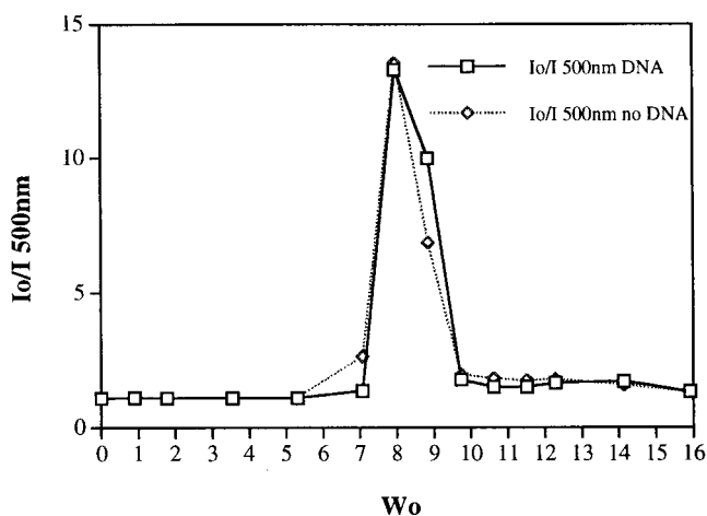
FIGURE 1 Inverse transmitted light ( I_0/I where I_0 is intensity of incident light and I is transmitted light) in relation to W_o . Light transmission was measured using a spectrophotometer at 500 nm of a w/o solution of C_{12}E_4 in 2,2,4-trimethylpentane at 20°C without DNA ( \diamond ) and in the presence of 11 \mu\text{g}/\text{mL} DNA ( \square ).
