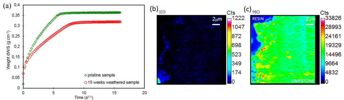
Fig. 1. (a) Imbibition kinetics measured on pristine and weathered limestone samples, (b) 32 S and (c) 16 O repartition mapping on the surface of the weathered limestone sample. Calcareous zone is on the right side and resin is on the left side of the map. The left side of the calcareous zone has been exposed to the fog.
