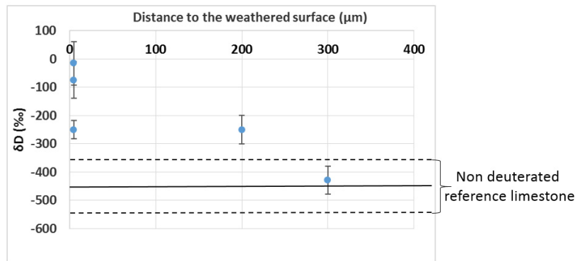
Fig. 2. Evolution of \delta\text{D} of water in pores as a function of the distance to the surface exposed to the deuterated fog.
