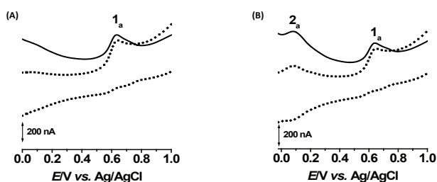
Figure 2. SW voltammograms obtained in pH 7.0 0.1 M phosphate buffer with a GCE in 25 \mu M resorcinol (A) first and (B) second scan; f = 25 Hz, \Delta E_s = 2 mV, v_{\text{eff}} = 50 mV s^{-1} , pulse amplitude 50 mV; I_t : total current; I_f : forward current, I_b : backward current.
