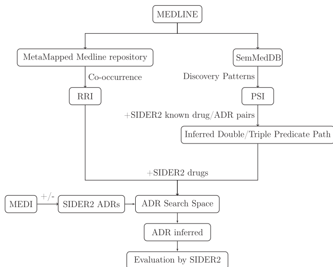
Fig. 5. Experimental design in the detection of SIDER2 known ADRs using LBD distributional semantic models.
