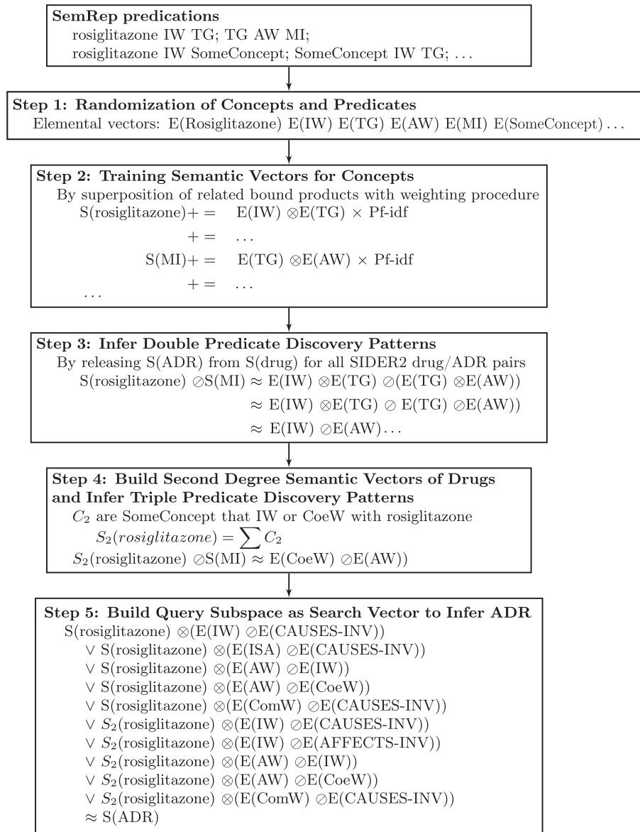
Fig. 4. Schematic representation of PSI training and inference process. triglycerides: TG; myocardial infarction: MI; INTERACTS_WITH: IW; COEXISTES_WITH: CoeW; ASSOCIATED_WITH: AW; COMPARED_WITH: ComW.
