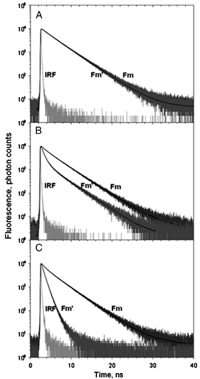
Fig. 3. Time correlated single photon counting analysis of chlorophyll fluorescence lifetime of LHCII complexes suspended in (A) high, (B) medium and (C) low detergent buffer (200, 20 and 6 \mu\text{M} , respectively) at pH 7.33 ( F_m ), pH 4.0 ( F_m' ).
