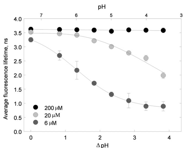
Fig. 4. Effect of pH on average fluorescence lifetime in native LHCII trimers suspended in high, moderate and detergent free buffer (final detergent concentrations of 200, 20 and 6 \mu\text{M} , respectively). Quenching was induced by the addition of HCl acid at a range of pH values between 7.33 and 3.5. Data represent average of four independent experiments \pm SE.
