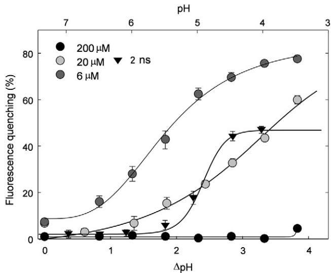
Fig. 2. Effect of pH on fluorescence quenching in native LHCII trimers suspended in 200, 20 and 6 \mu\text{M} of \beta\text{-DM} . Quenching was induced by the addition of HCl acid at a range of pH values between 7.33 and 3.5. Lines represent the curve fit using the Hill function. Data represent average of four independent experiments \pm SE.
