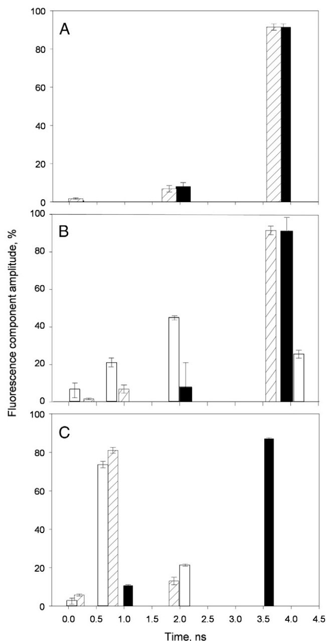
Fig. 5. Relative time resolved fluorescence lifetime component amplitudes of LHCII complexes suspended in 200 (A), 20 (B) and 6 (C) \mu\text{M} detergent buffer at pH 7.33 (black) and pH 4.0 (dashed). Open bars in (B) and (C) correspond to the components of pre-aggregated LHCII in 20 \mu\text{M} detergent at pH 7.33 and following acidification at pH 4.0, respectively. Data represent mean of four independent measurements \pm SEM.
