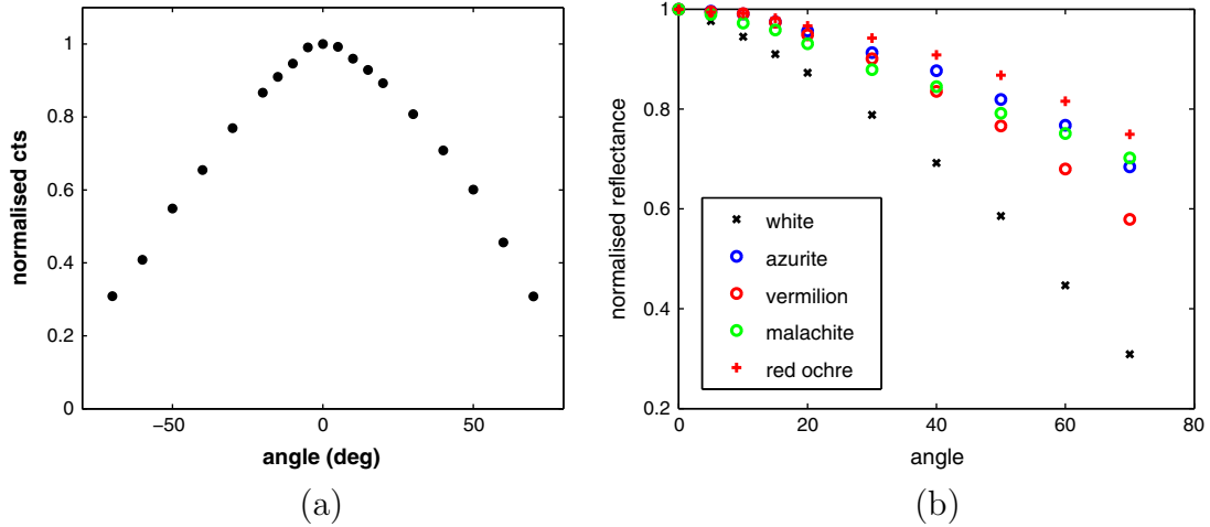
Fig. 7. (a) Normalised intensity measured through the 880 nm filter as a function of angle between the normal of the target surface and the optical axis of the camera at a distance of \sim 7 m for the matte Spectralon white standard; (b) a comparison of the angular dependence of the reflected intensity of light at 880 nm for different colour patches on a mock wall painting tile (picture shown in Fig. 10a) and the Spectralon white standard. (For interpretation of the references to colour in this figure legend, the reader is referred to the web version of this article.)
