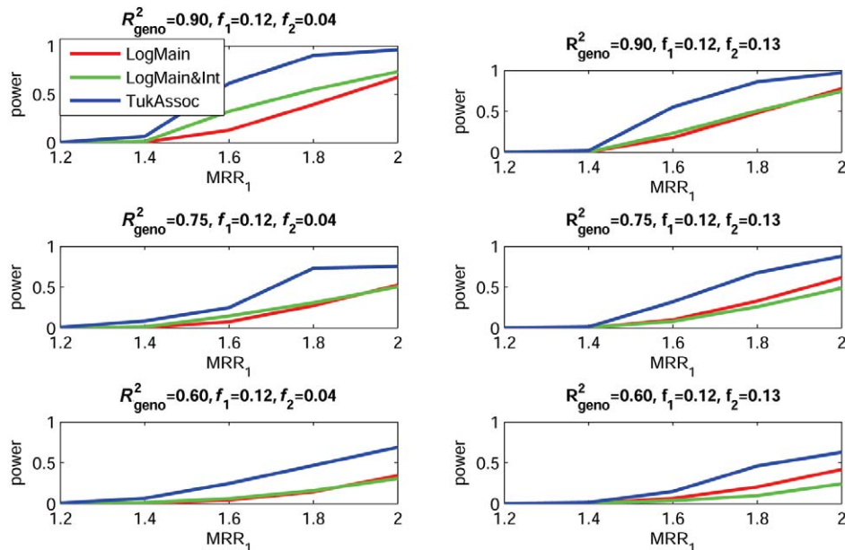
Figure 9. Empirical power, at \alpha = 0.0001 , to detect the association of the disease with candidate gene G_1 as a function of the MRR of the underlying causal SNP, S_1^* . The joint effect of casual SNPs in G_1 and G_2 follows the crossover model, with \phi_1 = 0.90 (see table 2). f_1 and f_2 denote minor-allele frequencies for causal SNPs in G_1 and G_2 , respectively, and R^2_{\text{geno}} denotes the value of multiple R^2 between the causal and marker loci within a gene.
