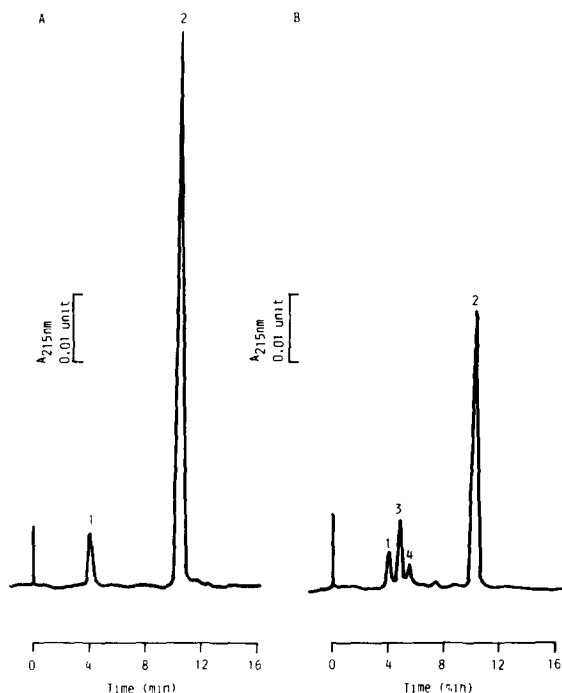
Fig.1. HPLC of culture filtrates. Columns were loaded with 25 \mu l culture filtrates. The absorbance scale was the same for both traces; the bar represents 0.01 A_{215} units. (A) Immediately after inoculation of acetate growth medium. (B) During exponential growth on acetate; the cell density was 221 \mu g dry wt/ml. Numbered peaks: 1, solvent front; 2, acetate; 3, 2-oxoglutarate; 4, citrate and isocitrate.
