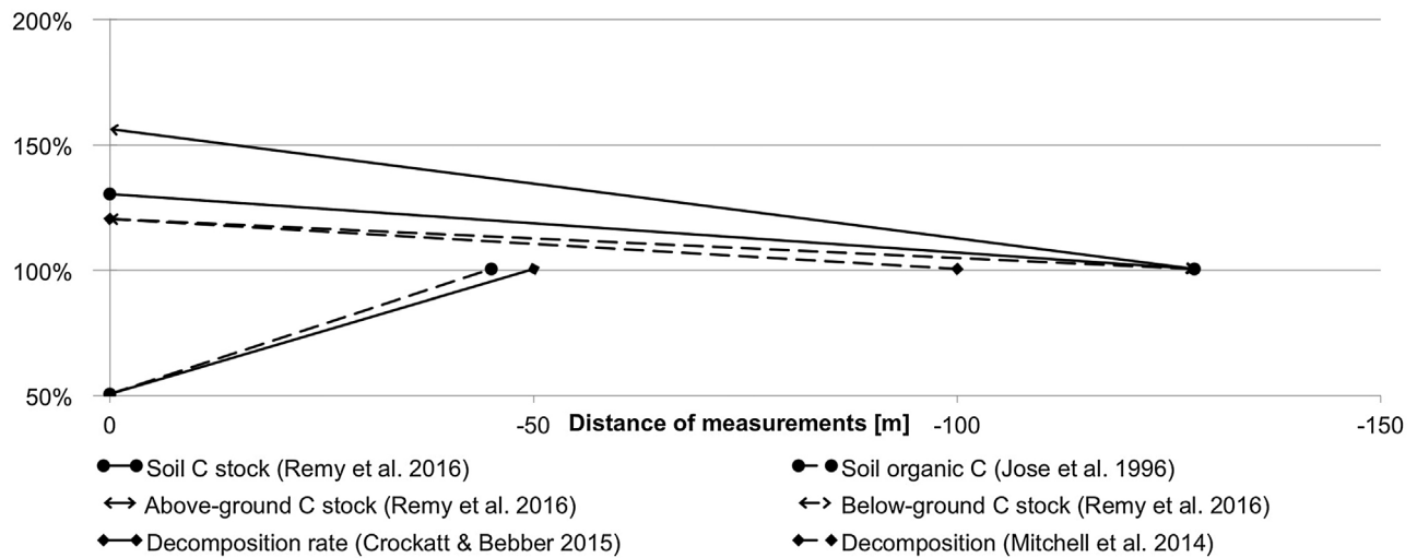
Fig. 5. Relative changes in the amount of carbon compounds and rates of related processes with respect to distance to the zero line (0 m) into forest transition zones.
