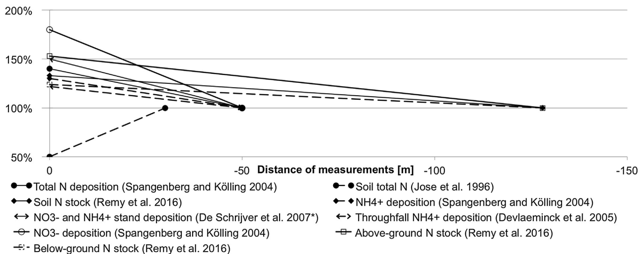
Fig. 6. Relative changes in the amounts of nitrogen compounds in soils in forest transition zones with respect to distance to zero line (0 m). *Median of reviewed articles.
