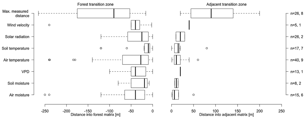
Fig. 4. Quartiles of influence in transition zones from the zero line between adjacent matrix and forest (left), and vice versa (right). Out of 76 studies concerning microclimate, 33 stated a distance. n = number of values reported for forest transition zones and adjacent transition zones. VPD = vapour pressure deficit. The box denotes 25–75% of the values with the median (bold) in it. The dashed bars are areas without outliers (small circles).
