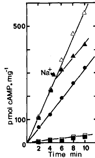
Fig. 4. Effect of \text{Na}^+ on the rate of cAMP synthesis. Washed membrane fractions were incubated for given times in the presence of GTP (0.1 mM) and with ( \Delta , \bullet , \circ ) or without ( \square , \blacksquare ) TSH (2.5 mU/ml). An \text{Na}^+ -free ATP regenerating system was present. \text{NaCl} (40 mM) was added to the incubation mixture at zero time ( \Delta , \bullet , \circ , \square , \blacksquare ) or after 5 min incubation in \text{Na}^+ -free medium ( \blacktriangle ).
