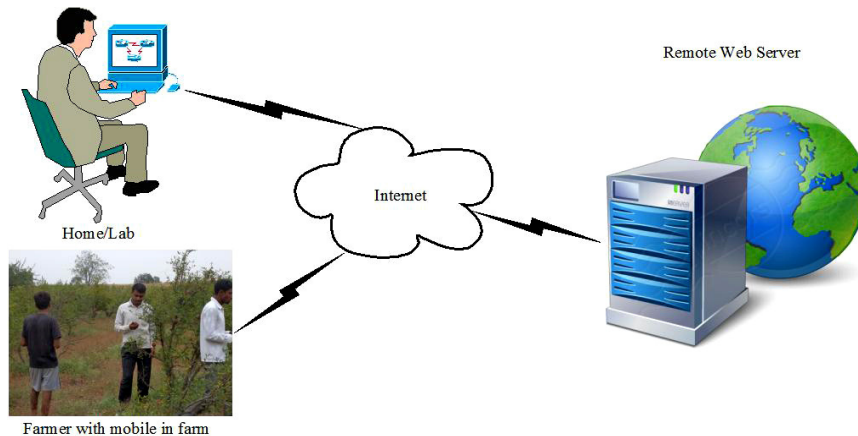
Fig. 2. System Architecture
