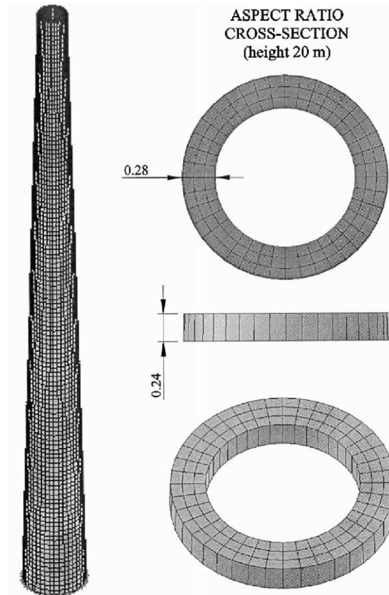
Fig. 9. Finite element model and aspect ratio used in the discretization (cross-section).
