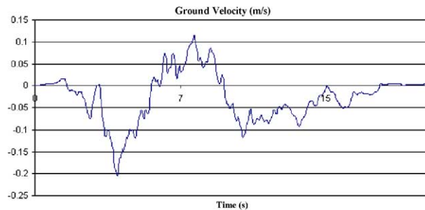
Fig. 5. Ground velocity.
