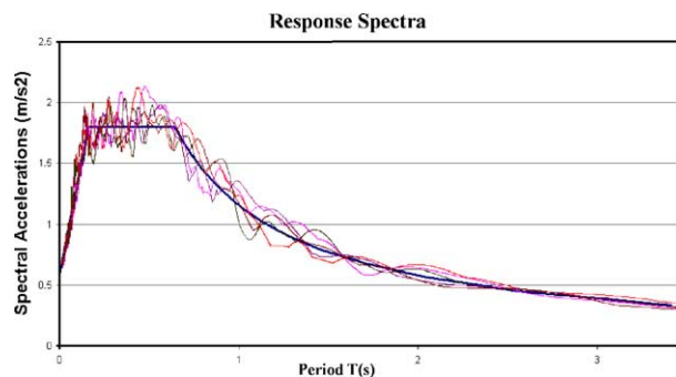
Fig. 7. Accelerations response spectra.
