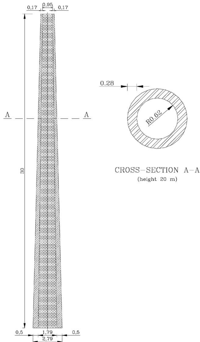
Fig. 8. Longitudinal section and cross-section at 20 m high.
