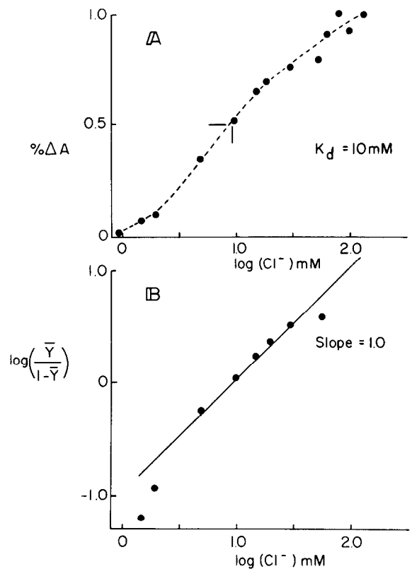
Fig. 4. Perturbation of catalase absorption upon chloride binding. Both %A (in A) and \bar{Y} (in B) represent normalized differences in absorbance at 405 nm minus 390 nm.
