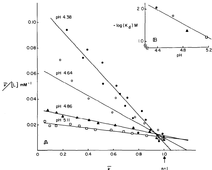
Fig.5. Binding of chloride to catalase at different pH values. Dissociation constants, derived from Scatchard plots (in A), are plotted versus pH (in B). L equals chloride concentration, and \bar{v} represents the molar ratio of bound ligand to total catalase heme.
