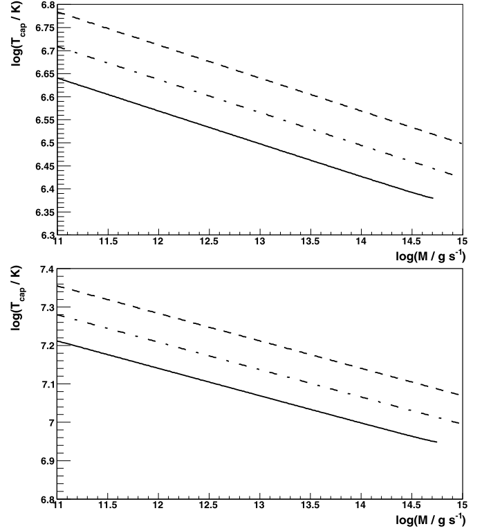
Fig. 4. The surface temperature of the hot polar cap region as a function of the Bondi accretion rate for selected values of the magnetic moment of the neutron star fixed on 10^{26} \text{ G cm}^3 (solid curve), 3 \times 10^{26} \text{ G cm}^3 (dashed) and 10^{27} \text{ G cm}^3 (dot-dashed) and the millisecond pulsar with the period equal to 1.6 ms (upper panel). The case of the classical pulsar with the period of 300 ms and the magnetic moment of the neutron star fixed on 10^{30} \text{ G cm}^3 (solid curve), 3 \times 10^{30} \text{ G cm}^3 (dashed) and 10^{31} \text{ G cm}^3 are shown in the bottom panel.
