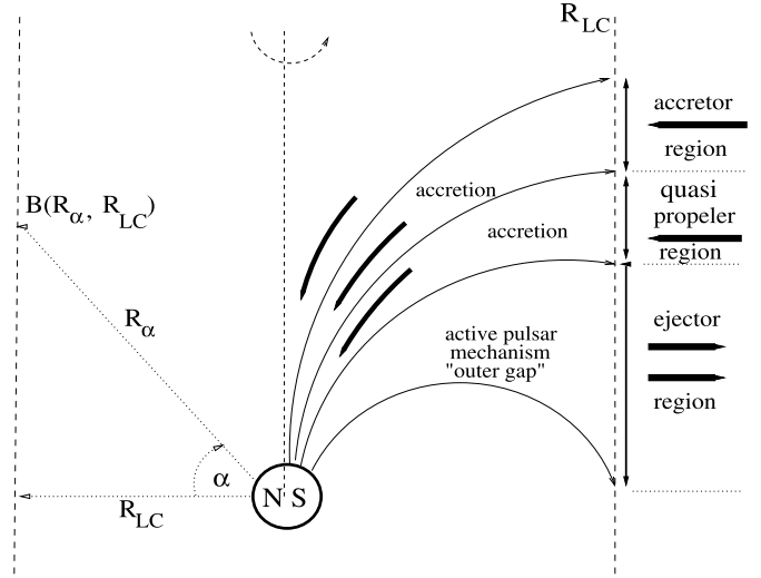
Fig. 1. Schematic representation of the hybrid accretion scenario in which a part of the magnetosphere is still in the ejector mode and a part of the pulsar magnetosphere is already able to accrete the matter distributed quasi-spherically. Since a part of the magnetosphere, close to the rotational plane of the pulsar, is free of matter, the outer gap acceleration model for the radiation processes (Cheng et al., 1986) can still operate in this part of the magnetosphere which is connected to the magnetosphere outside the light cylinder radius in the ejector stage. We define the critical angle, \alpha_{\text{cr}} , as the angle \alpha which separates a part of the pulsar magnetosphere in the ejector region from a part in the accretor region. The angle \alpha_{\text{cr}} is determined by the condition that the magnetic field energy density, at the light cylinder ( R_{\text{LC}} ) and at the distance R_{\alpha} from the center of the neutron star, is equal to the free fall kinetic energy of accreting matter (see Eq. (3)). Then, the pulsar magnetosphere is composed of two parts. The accretion occurs with almost free fall velocity along the magnetic field lines which are connected to accretor region. The accretion occurs with the velocity significantly reduced from the free fall velocity, due to the partial balance of the gravitational force by the centrifugal force, along the magnetic field lines which lay in the region called quasi-propeller.
