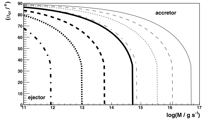
Fig. 2. The value of the critical angle as a function of different accretion rates (calculated for the case of quasi-spherical accretion) for a few selected NS rotational periods, P_{\text{ms}} = 1.6 ms (solid curve), 3 ms (dashed), 5 ms (dotted), and 10 ms (dot-dashed). The ejector mode is expected for the low accretion rates and small angles \alpha (below thick curves). The accretor mode is expected for the angle \alpha_{\text{cr}} above the thick curves. The thin curves separate the quasi-propeller and accretor modes of accretion onto the NS surface. The magnetic moment of the neutron star is fixed on 10^{26} \text{ G cm}^3 .
