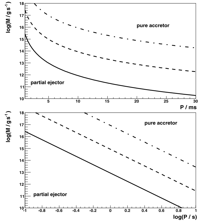
Fig. 3. The parameter space (the pulsar period versus the Bondi accretion rate) for the partial ejector mode and only (pure) accretor mode for the case of millisecond pulsars (upper panel) and classical pulsars (bottom panel). The magnetic moment of the NS is equal to \mu_{\text{NS}} = 10^{26} \text{ G cm}^3 (solid curve), 10^{27} \text{ G cm}^3 (dashed curve), and 10^{28} \text{ G cm}^3 (dot-dashed curve) in the upper panel and for 10^{30} \text{ G cm}^3 (solid), 10^{31} \text{ G cm}^3 (dashed), and 10^{32} \text{ G cm}^3 (dot-dashed) in the bottom panel.
