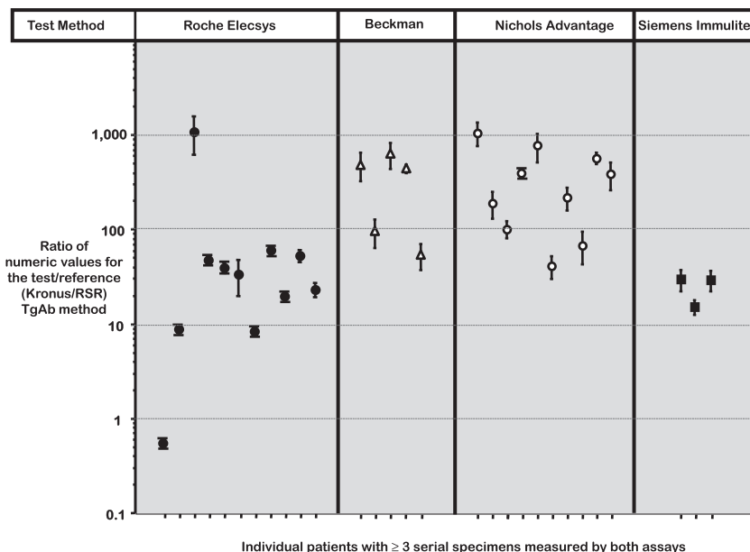
Fig. 1. Mean \pm sd of the ratios between the numeric values (kIU/L) reported by a test method, Roche (solid circles); Beckman (open triangles); Nichols Advantage (open circles) or Siemens Immulite (closed squares), divided by the numeric values of the reference method (Kronus/RSR) for individual DTC patients with 3 or more serial serum specimens sent for TgAb testing as a component of serial serum Tg monitoring over a period of 1–4 years.
