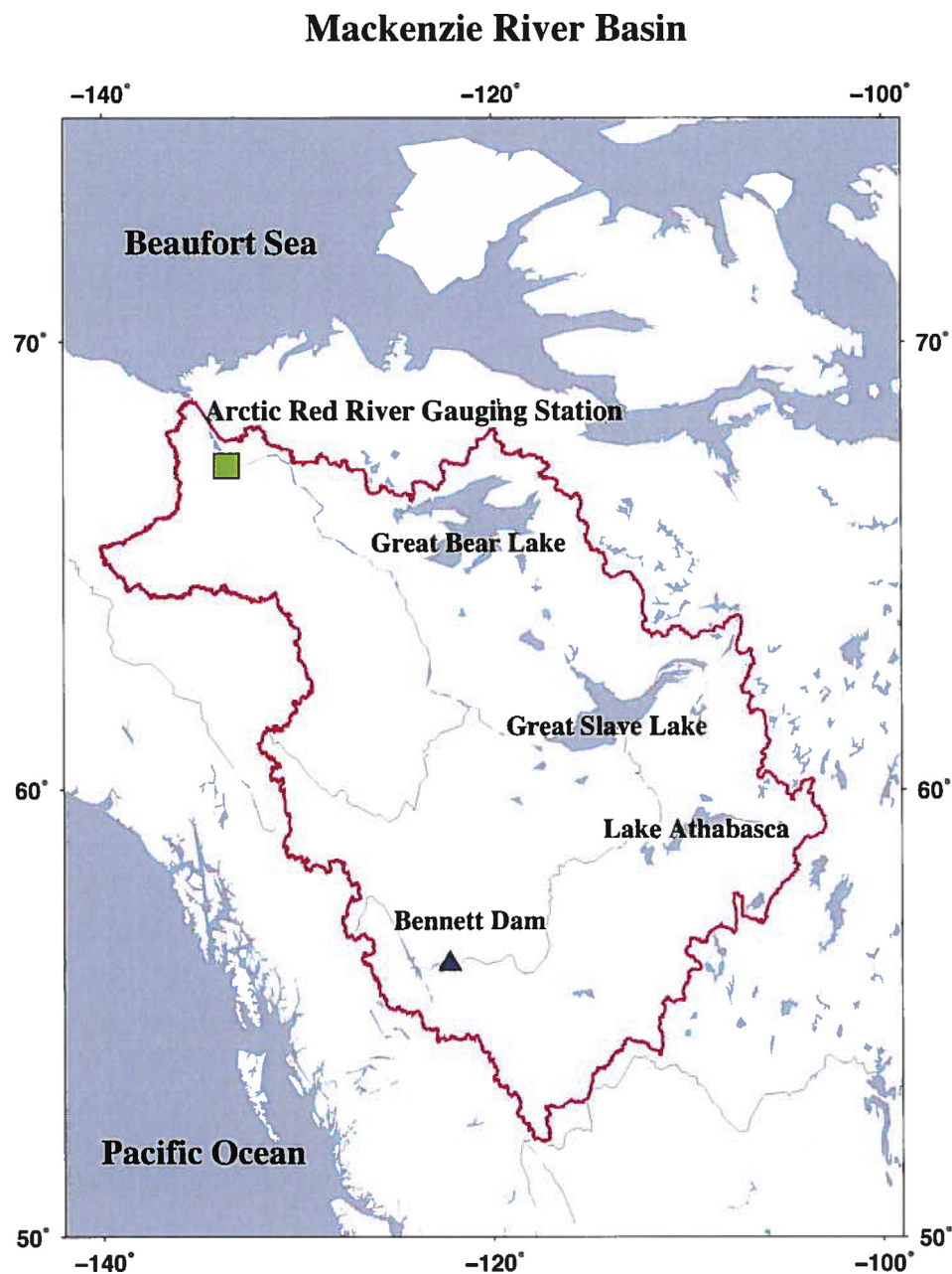
Fig. 1. The Mackenzie River system, including major sub-basins and locations of large lakes, reservoir, and the Arctic Red River gauging station near the basin outlet. (For interpretation of the references to colour in this figure legend, the reader is referred to the web version of this article.)
