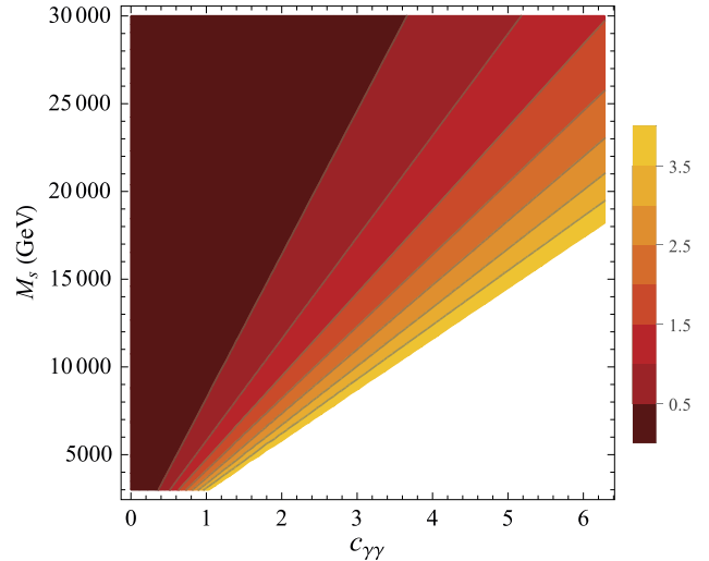
Fig. 1. Contours of constant partial width \Gamma_{\gamma\gamma} . The color encoded scales are in GeV. (For interpretation of the references to color in this figure legend, the reader is referred to the web version of this article.)
