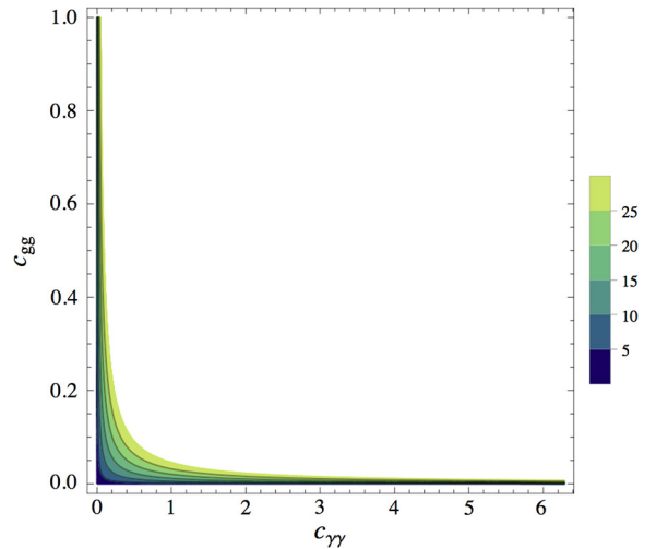
Fig. 4. Contours of constant string scale M_s for best fit of diphoton cross section ( \sigma_{\text{LHC13}} = 5 fb) produced via gluon fusion ( M_\phi \simeq 750 GeV, \sqrt{s} = 13 TeV). The color encoded scales are in TeV. The different panels correspond to \Gamma_{\text{total}} = 45, 10, 0.1 GeV, downwards. (For interpretation of the references to color in this figure legend, the reader is referred to the web version of this article.)
