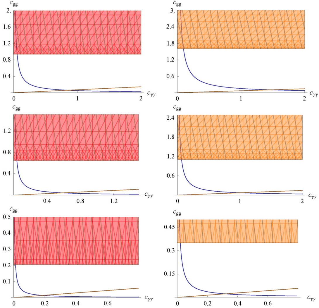
Fig. 5. Allowed parameter space on the c_{gg} vs c_{\gamma\gamma} plane for M_s = 7 TeV (left) and M_s = 12 TeV (right). The blue curves indicate the best fit of diphoton cross section ( \sigma_{\text{LHC13}} = 5 fb) for M_s = 7 TeV (left) and M_s = 12 TeV (right). The red and orange shaded regions are excluded at 95% CL by null results on dijet searches. The slanted (brown) curve determines the transition between c_{gg} and c_{\gamma\gamma} dominance at production. Gluon fusion dominates above this curve. Results for three possible total widths are exhibited in the vertical columns, \Gamma_{\text{total}} = 45, 10, 0.1 GeV, downwards. (For interpretation of the references to color in this figure legend, the reader is referred to the web version of this article.)
