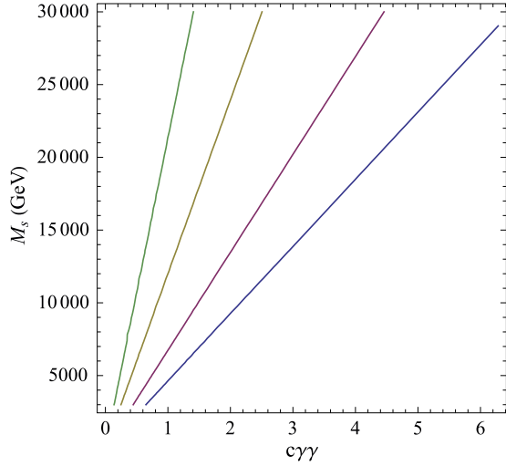
Fig. 2. Best fit contours of diphoton cross section \sigma_{\text{LHC13}} \sim 5 fb produced via photon fusion \gamma\gamma \rightarrow \phi \rightarrow \gamma\gamma . The four lines (blue, red, yellow, green) are for \Gamma_{\text{total}} = 45, 10, 1.0, 0.1 GeV, respectively. (For interpretation of the references to color in this figure legend, the reader is referred to the web version of this article.)
