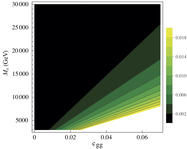
Fig. 3. Contours of constant partial width \Gamma_{gg} . The color encoded scales are in GeV. (For interpretation of the references to color in this figure legend, the reader is referred to the web version of this article.)
