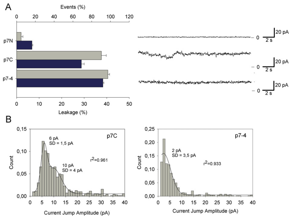
Fig. 4. Pore-forming activity of p7N, p7C and p7-4 peptides in ER-like planar bilayers and vesicles at pH 5.0. A Left: Comparison of the ability to form channels in planar bilayers (light gray) with leakage induced in LUVs by the addition of p7 peptides to a peptide-to-lipid mole ratio of 1:250 (dark gray). Right: Representative traces of IC activity. B ) Histograms of the current jump amplitude measured for the active p7C and p7-4 peptides. The histograms have been fitted to two Gaussian peaks (left panel) and single Gaussian peak (right panel), respectively.
