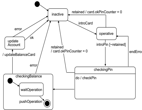
Fig. 5. Statechart of Card class.
