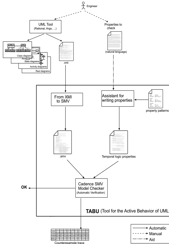
Fig. 1. Tool architecture
