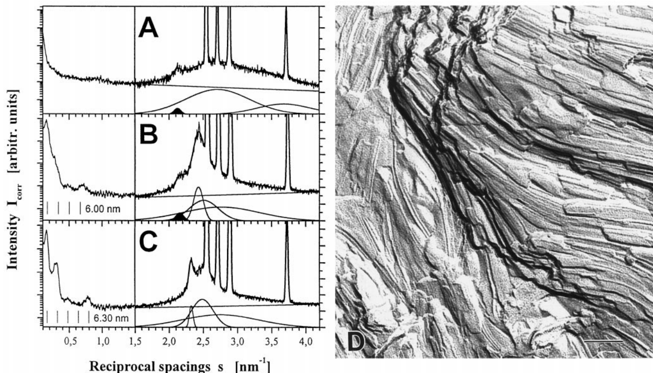
FIGURE 2 Combined small-angle and wide-angle x-ray diffractograms of ( A ) the peptide in aqueous buffer, ( B ) B18 reconstituted with DMPC (lipid/peptide ratio of 10:1), and ( C ) multilamellar DMPC liposomes at -10°C. Deconvolution of the wide angle diffraction regions reveals a characteristic \beta -sheet spacing of 0.47 nm for the peptide ( shaded peaks ), which proves that it forms amyloid fibrils both in buffer ( A ) and in the presence of the lipid ( B ). The bilayer repeat distance is slightly decreased in the presence of B18, as indicated by the arrays of lines in the small-angle regions of B and C . The deformed hexagonal lipid packing in the gel state is also affected, as seen by the positions and widths of the deconvoluted peaks in the wide-angle regions of B and C . The lipid/peptide sample used for B was also characterized by EM ( D ), revealing a high density of parallel structures that are attributed to peptide fibrils. The shadowing direction of this and all further EM images is oriented from bottom to top, and the bar represents 100 nm.
