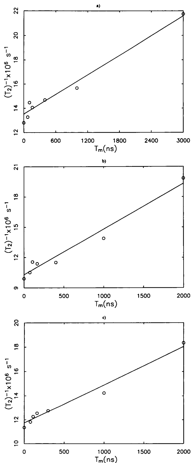
FIGURE 10 The plot of apparent homogeneous linewidths, T_2 values as a function of the mixing time, T_m , for CSL/POPC at three different temperatures: (a) 50^\circ\text{C} ; (b) 60^\circ\text{C} ; and (c) 70^\circ\text{C} .
