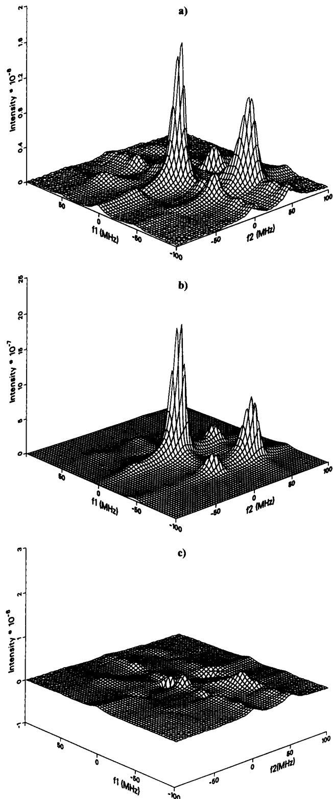
FIGURE 2 Plots of (a) experimental, (b) best NLLS simulation, and (c) the difference between a and b for a 2D ELDOR spectrum from CSL/POPC.
