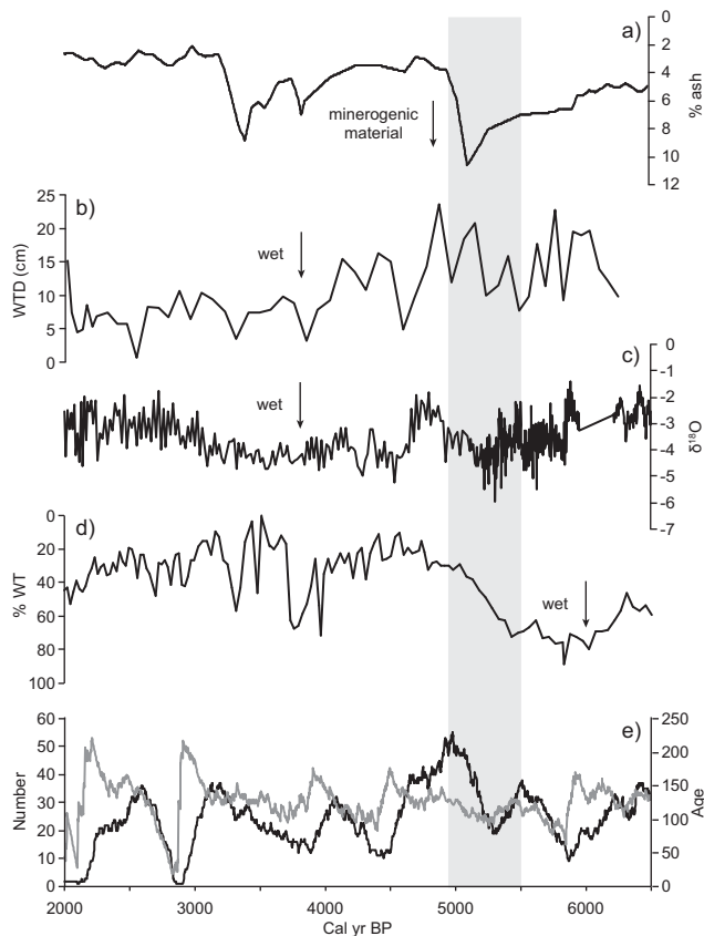
Fig. 7. Palaeoclimatic records from Ireland, 6.5–2 ka. a) Loss-on-ignition records Caisleán peat cores, Achill Island, western Ireland (Caseldine et al., 2005); b) Testate amoebae-based water table reconstruction (ACCROTELM transfer function) from Derragh Bog, central Ireland (Langdon et al., 2012); c) \delta^{18}\text{O} from speleothem CC3, Crag Cave, southwest Ireland (McDermott et al., 2001); d) \text{CaCO}_3 record, expressed as a weight percentage, from Inis Oírr, western Ireland (Schettler et al., 2006); e) Northern Irish dendro-dated bog oak population (black) and average age (grey) (Turney et al., 2005). The period 5.5–4.95 ka is highlighted in grey.
