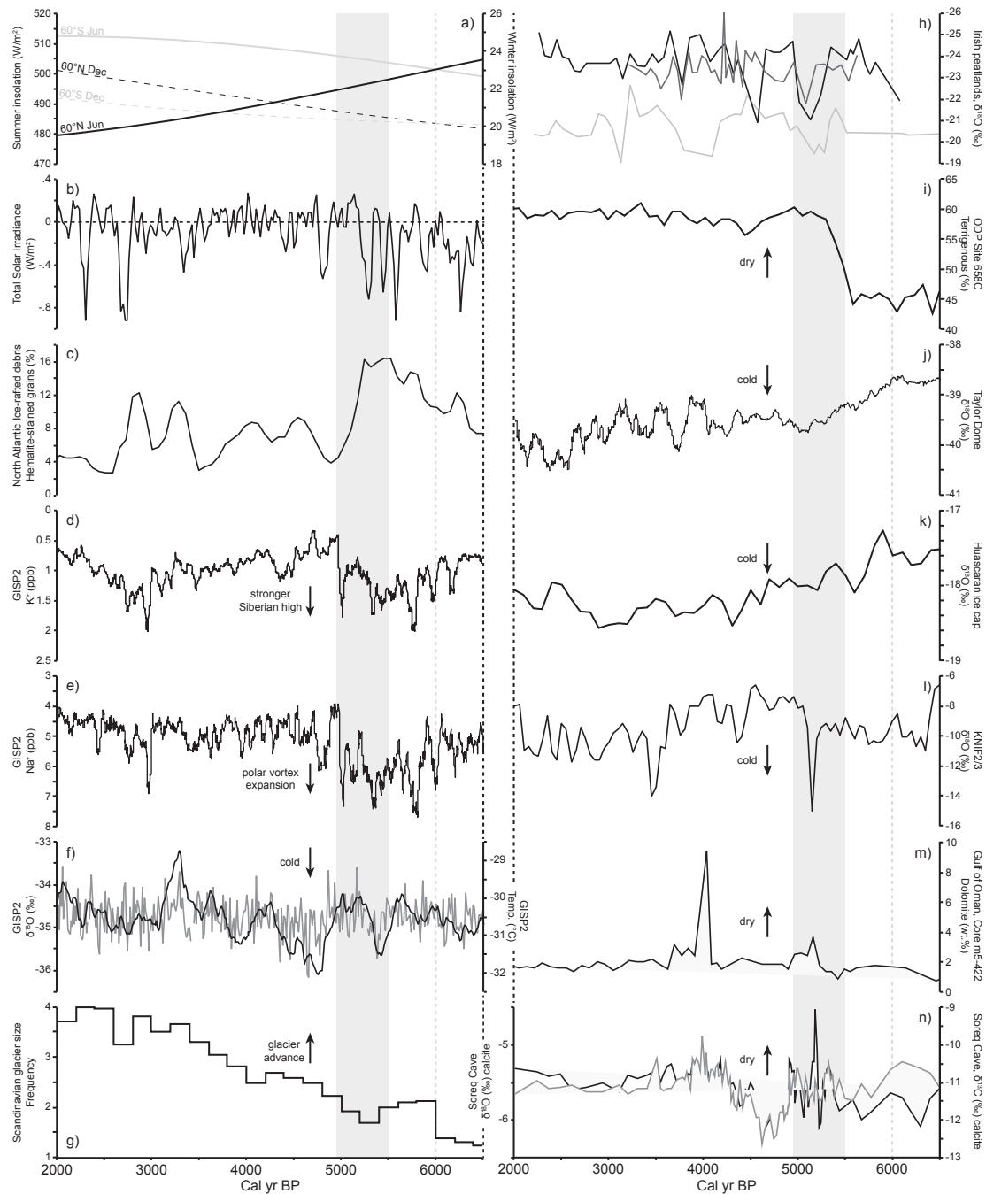
Fig. 8. Global palaeoclimate records, 6.5 – 2 ka. a) Summer (solid) and winter (dashed) insolation from 60°N (black) and 60°S (grey) (Berger and Loutre, 1991); b) Total solar irradiance based on ^{10}\text{Be} ^{14}\text{C} in tree rings and polar ice cores (Steinhilber et al., 2012); c) North Atlantic hematite-stained grains record (stacked cores: MC52, V29191, MC21 and GGC22) (Bond et al., 2001); d) Potassium ion ( \text{K}^+ ) content of GISP2 ice core (Mayewski et al., 1997); e) Sodium ion ( \text{Na}^+ ) content of GISP2 ice core (O'Brien et al., 1995); f) Temperature over Greenland (GISP2) (Alley, 2000) derived from \delta^{18}\text{O} (Stuiver et al., 1995); g) Frequency-distribution histogram (100-yr interval) of Scandinavian glacier-size variations (Nesje, 2009); h) \delta^{18}\text{O}_{\text{cellulose}} data from Sluggan Moss (black), Fallahogy Bog (mid-grey) and Raheenmore (light grey) (this study); i) Terrigenous (aeolian) sediment percentage record from ODP Site 658C, West Africa (Demenocal et al., 2000); j) \delta^{18}\text{O} record from Taylor Dome ice core, Antarctica (Steig et al., 2000); k) \delta^{18}\text{O} record for Huascarán ice cap, Peru (Thompson et al., 1995); l) \delta^{18}\text{O} record for Kilimanjaro ice-core, Tanzania (Thompson et al., 2002); m) Percentage by weight of dolomite of Mesopotamian origin in marine sediments from the Gulf of Oman (Cullen et al., 2000); n) \delta^{18}\text{O} (black) and \delta^{13}\text{C} (grey) from a speleothem in Soreq Cave, Israel (Bar-Matthews et al., 2003).
