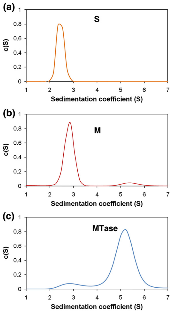
Fig. 2. SV analysis of the MTase and its subunits. The c(s) distribution plots are shown for (a) S^{NT} at 25 \mu\text{M} , (b) M at 6 \mu\text{M} and (c) M.EcoR124I NT at 2.6 \mu\text{M} . All experiments were performed at 30,000 rpm (in a Beckman Coulter An50 Ti analytical rotor), at 10 °C in buffer A, scanning every 12 min, at 280 nm.
