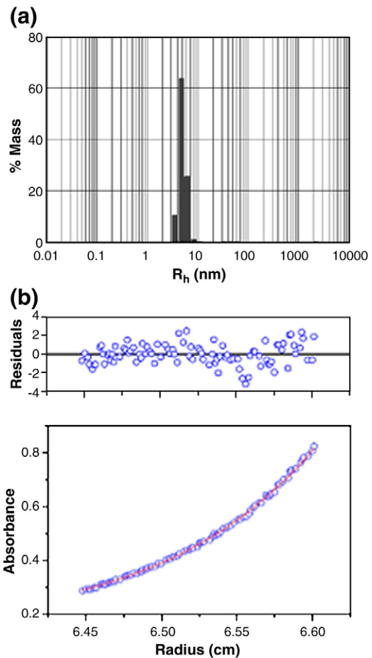
Fig. 3. (a) DLS of M.EcoR124I NT at a concentration of 5 \mu\text{M} at 10 °C. A hydrodynamic radius of 5 nm with a polydispersity of 0.87 nm (7.4%) was obtained. (b) SE of M.EcoR124I NT . Shown is an example fit from data collected at 8500 rpm (using a Beckman Coulter An50 Ti analytical rotor), scanned at 276 nm (after 21 h), at a concentration of 5 \mu\text{M} at 10 °C. The data were fitted to a single ideal species model and yielded an apparent M_r of 162,100. The top panel shows the residual error between the fitted and experimental values.
