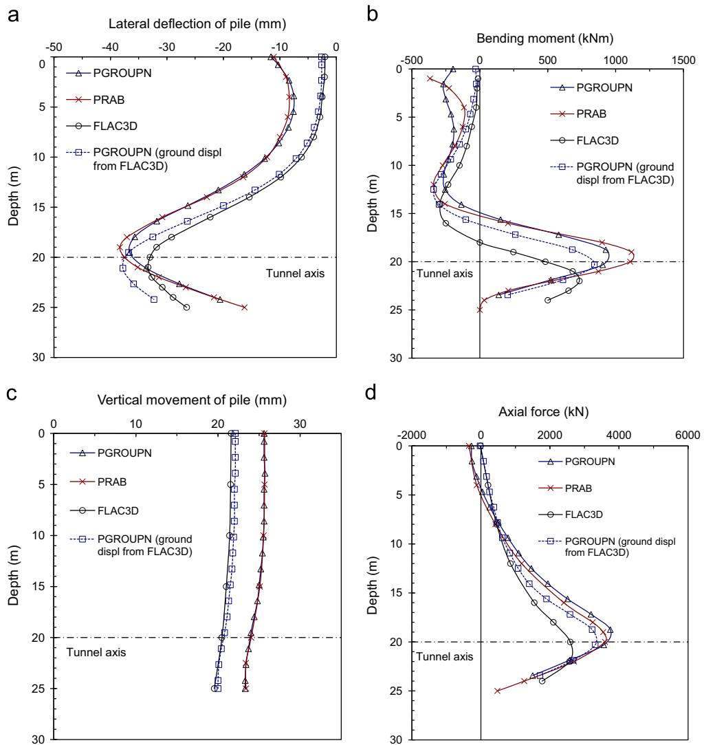
Fig. 8. Comparison of pile-group responses for front pile.
