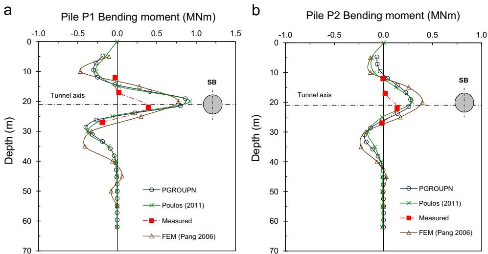
Fig. 16. Measured and computed bending moment distributions for (a) pile P1 and (b) pile P2.
