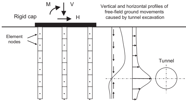
Fig. 1. BEM schematisation of the problem.
