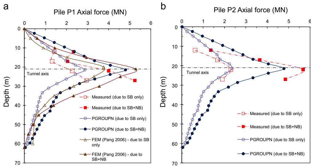
Fig. 19. Measured and computed axial force distributions for (a) pile P1 and (b) pile P2.
