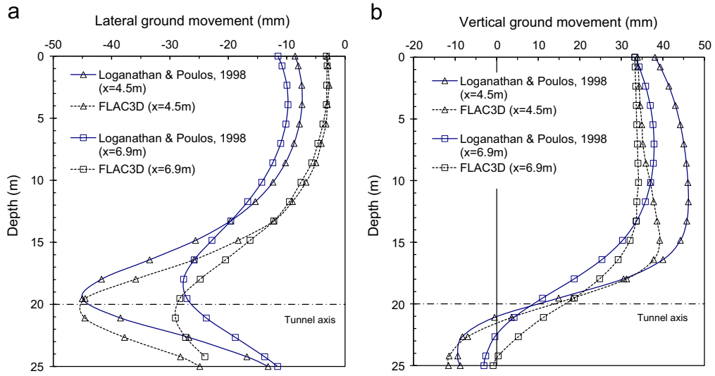
Fig. 7. Comparison of computed free-field ground movements.
