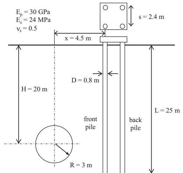
Fig. 4. Pile-group problem analysed.
