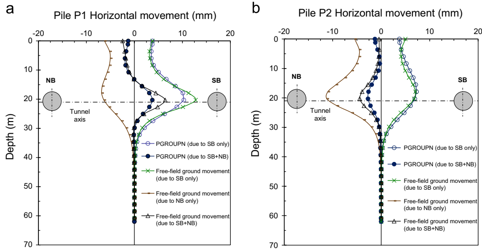
Fig. 18. Horizontal movement profiles for (a) pile P1 and (b) pile P2.
