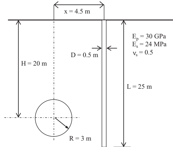
Fig. 2. Single-pile problem analysed.
