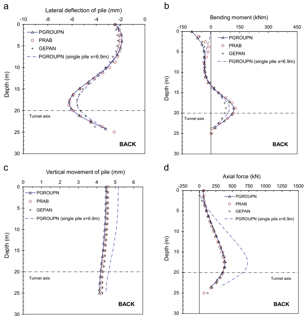
Fig. 6. Comparison of pile-group responses for back pile.
