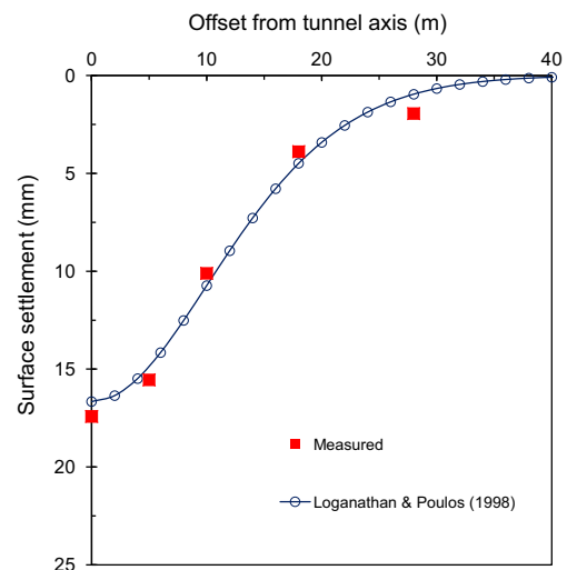
Fig. 12. Measured and computed free-field surface settlements.
