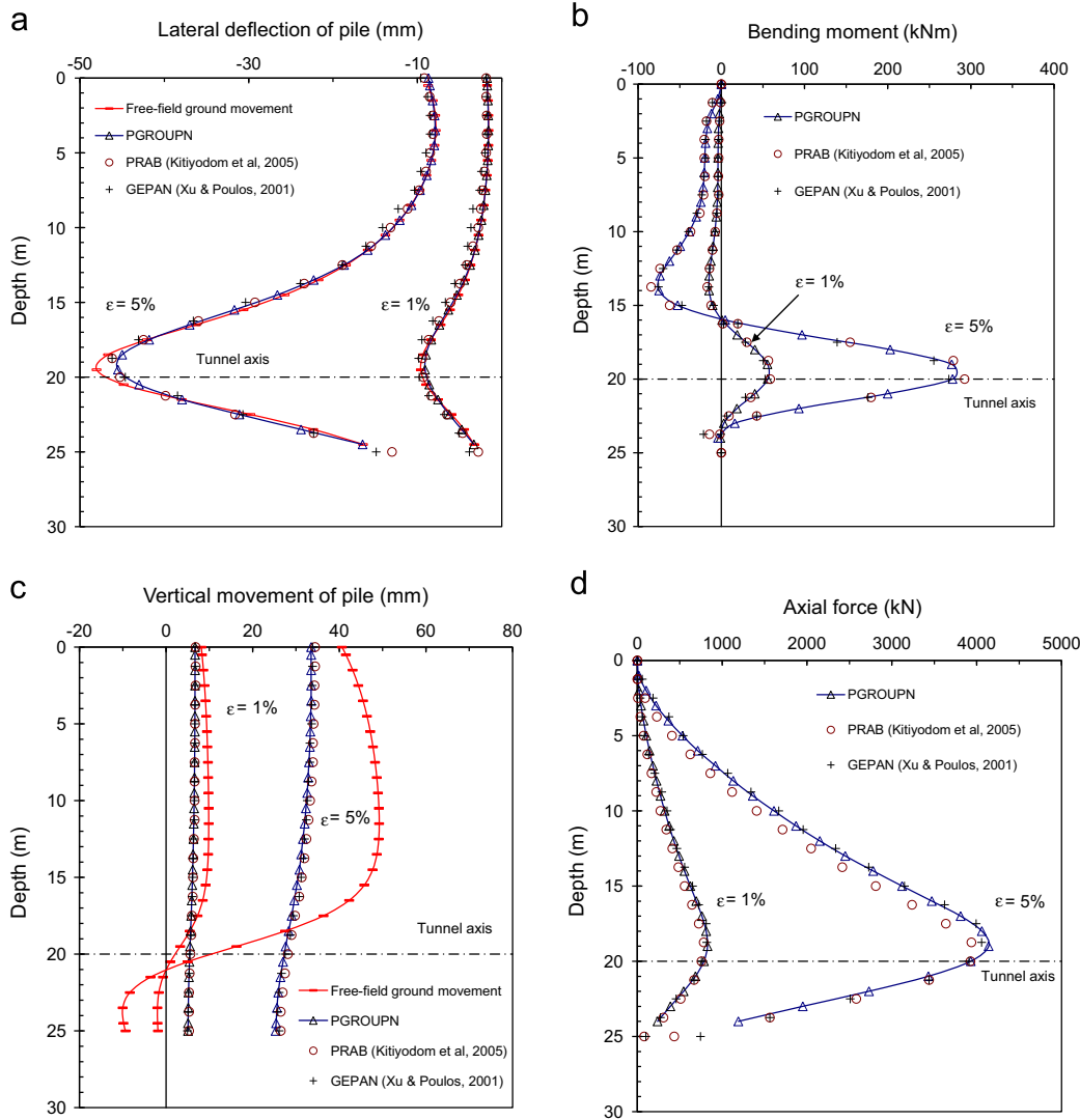
Fig. 3. Comparison of single-pile responses.
