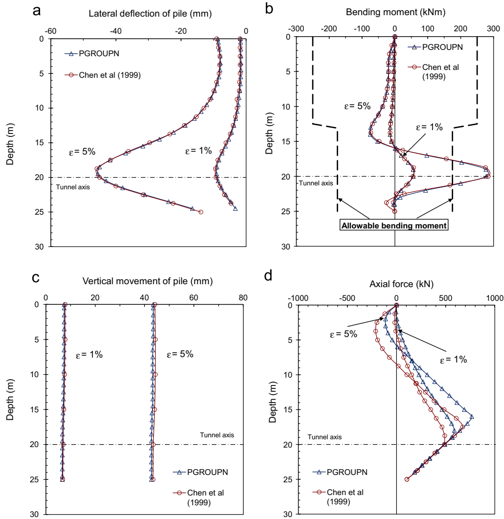
Fig. 9. Comparison of single-pile responses.
