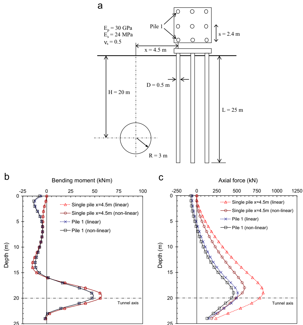
Fig. 10. Pile-group problem analysed and PGROUPN predictions.
