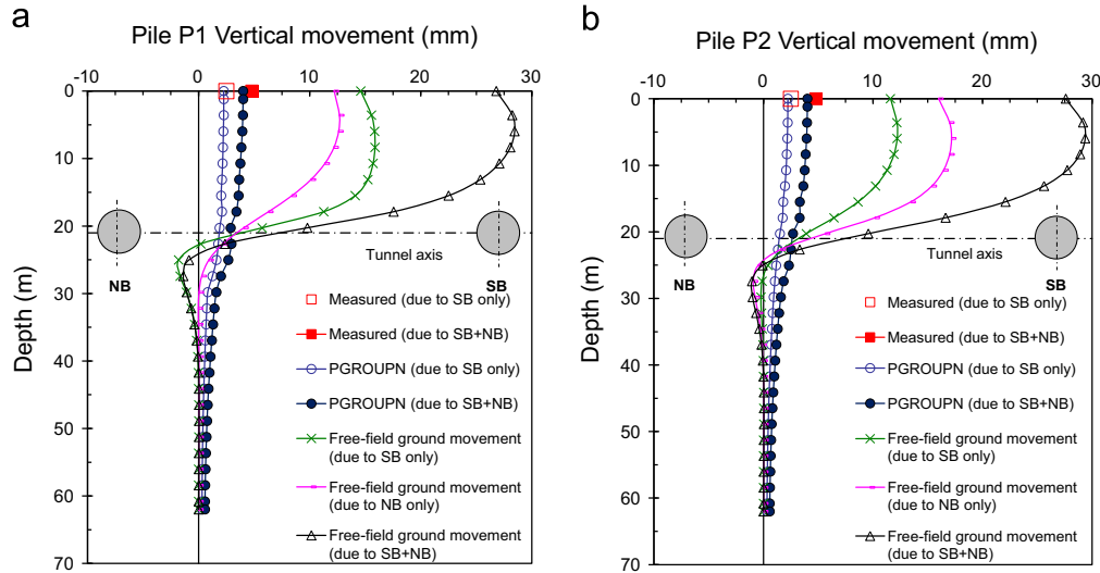
Fig. 17. Vertical movement profiles for (a) pile P1 and (b) pile P2.
