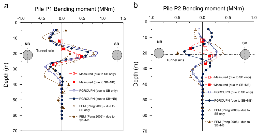
Fig. 20. Measured and computed bending moment distributions for (a) pile P1 and (b) pile P2.
