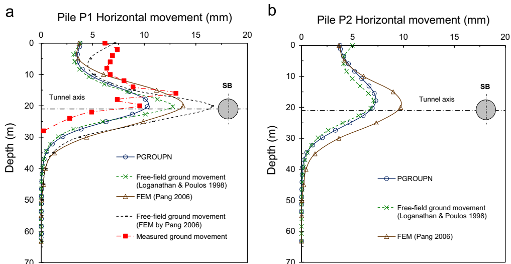
Fig. 14. Horizontal movement profiles for (a) pile P1 and (b) pile P2.
