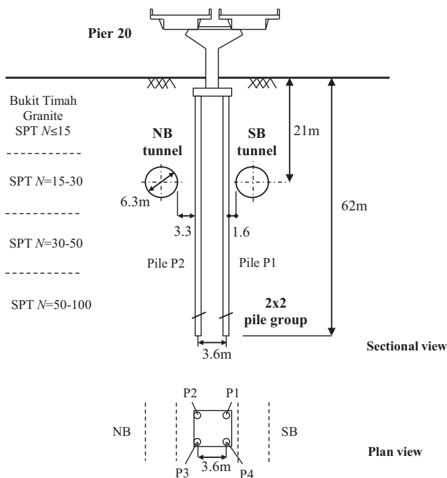
Fig. 11. Pile and tunnel layout at Pier 20 (after Pang, 2006).
