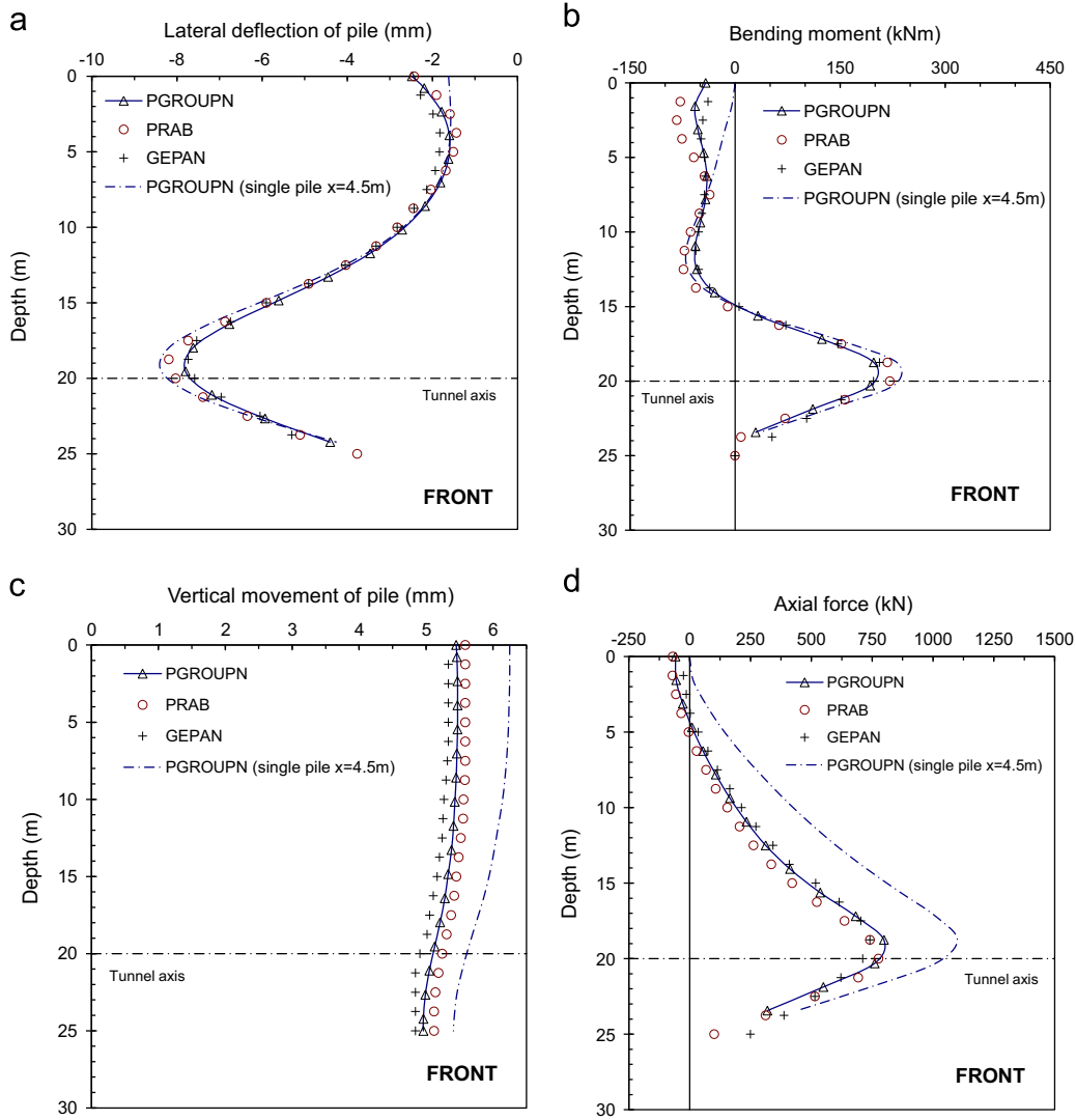
Fig. 5. Comparison of pile-group responses for front pile.
