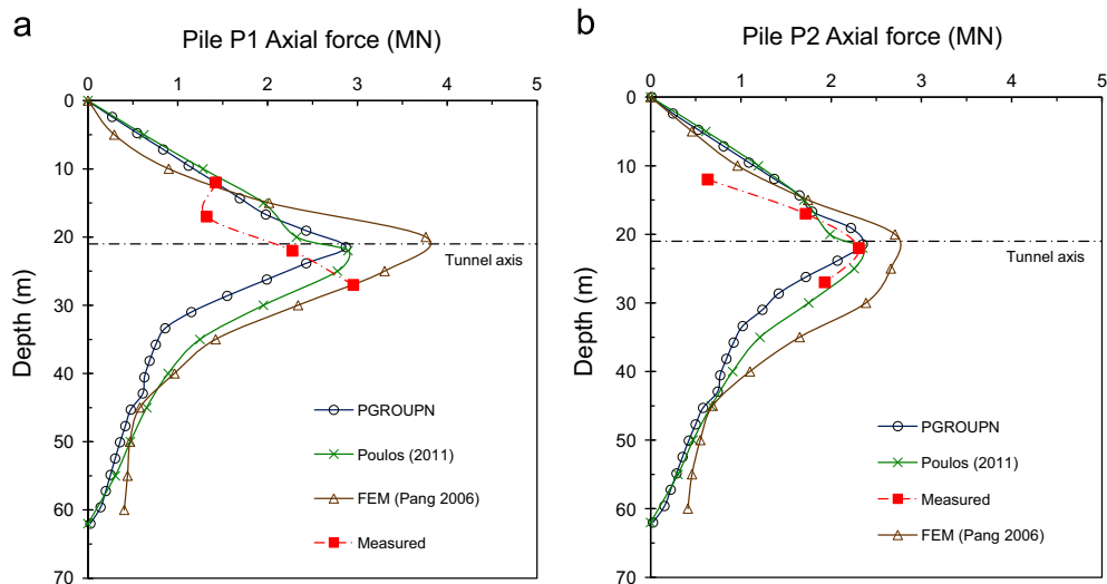
Fig. 15. Measured and computed axial force distributions for (a) pile P1 and (b) pile P2.
