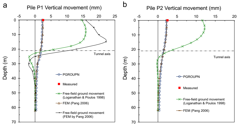
Fig. 13. Vertical movement profiles for (a) pile P1 and (b) pile P2.
