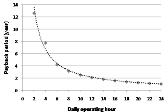
Fig. 6. Simple payback period for LED T8 over fluorescent T8.
