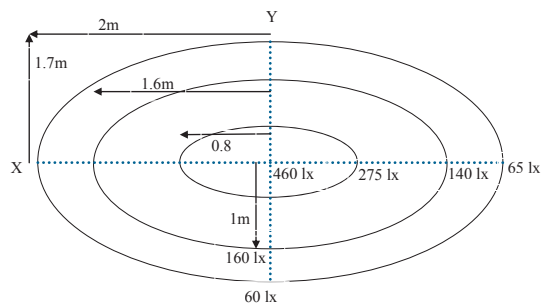
Fig. 3. Photometry lighting system of LED tube.
