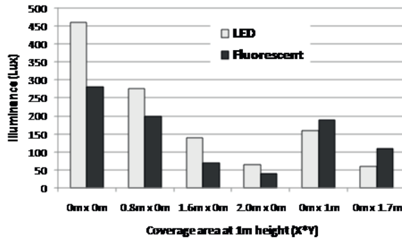
Fig. 5. Summary of photometry lighting system comparison.
