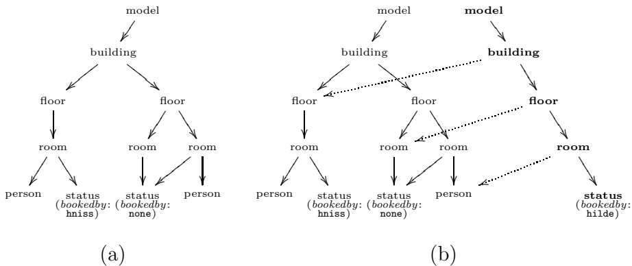
Fig. 2. Reusing unchanged nodes (dotted arrows indicate reuse; bold text indicate the newly constructed path).
