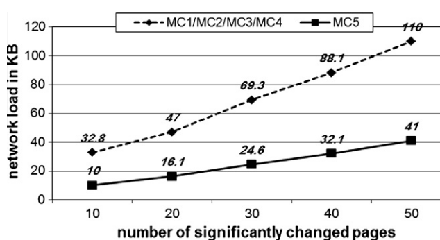
Figure 6 Number of bytes transferred through the network when different number of pages are added or significantly changed.
