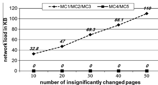
Figure 7 Number of bytes transferred through the network when different number of pages are insignificantly changed.
