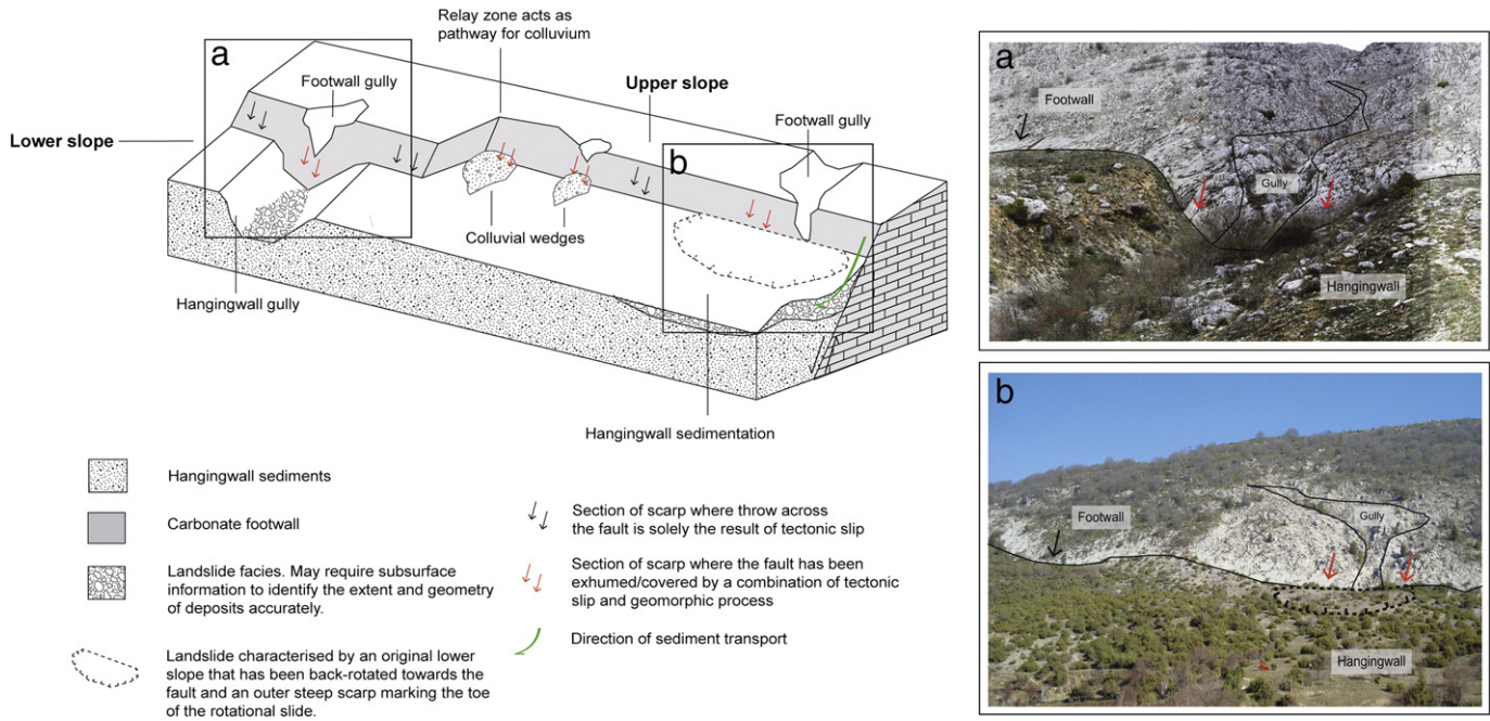
Fig. 9. Summary of processes contributing to scarp exposure in the central Apennines.
