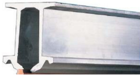
Fig. 2. Rigid overhead catenary. It clamps the copper wire that contacts the pantograph
