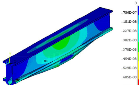
Fig. 3. Integration of the project with other disciplines. Finite elements analysis of the static problem [10]
