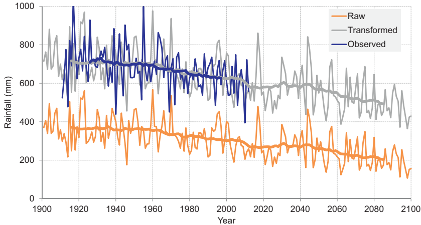
Fig. 6. A comparison of observed (blue), simulated (MPI-ESM-LR, orange) and transformed (gray) annual SWWA rainfall. 31-year running average values are indicated.
