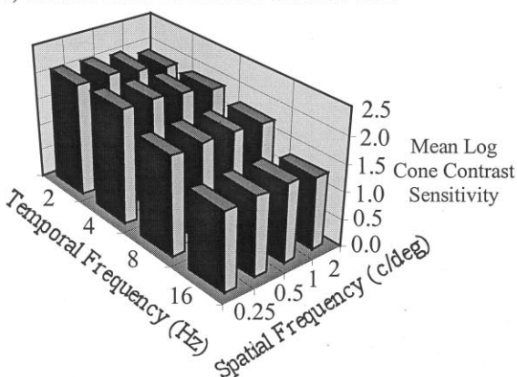
Fig. 1. Geometric means obtained from 21 subjects tested at each of 16 spatial-temporal frequencies, for three different stimulus conditions. (A) Green/red equiluminance. Here, a log G/R ratio of zero denotes V_z equiluminance. Across all conditions, subjects tended to require more green to match the red, as evidenced by mean log G/R ratios greater than zero. We do not attribute any significance to this, but rather believe it is a simple consequence of the particular stimulus parameters used in our experiments (i.e. size and placement of stimuli, background chromaticity, etc.). (B) Luminance contrast sensitivity. (C) Chromatic contrast sensitivity. In order to facilitate comparison between spatial-temporal frequency conditions, standard deviations are not plotted. Standard deviations were, on average, 0.02 log units for the equiluminance data, 0.13 log units for luminance data, and 0.15 log units for chromatic data.
