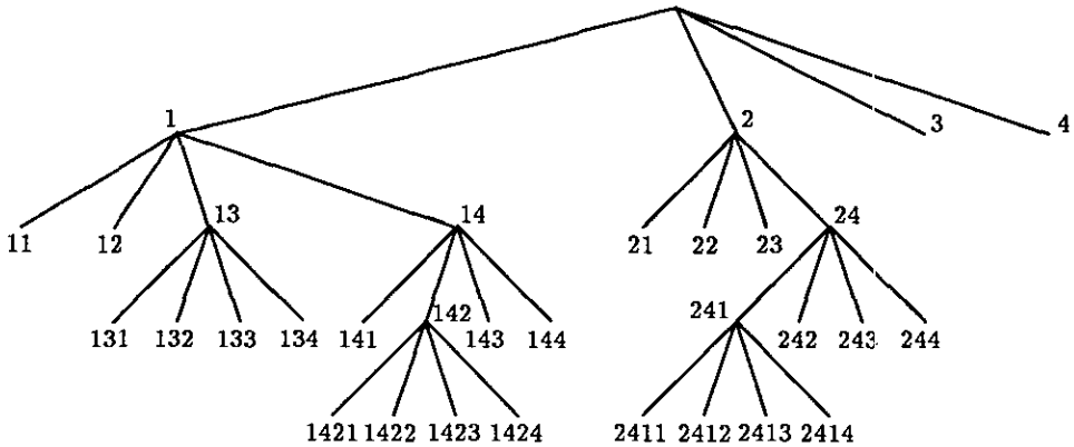
Figure 2. The Four Queens Search Tree
