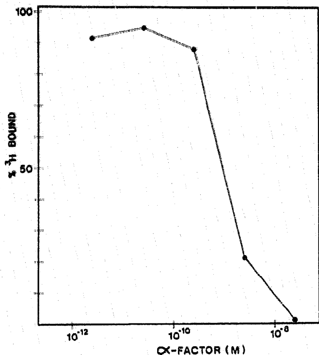
Fig. 1. Inhibition of [ 3 H]α-factor binding. α-Cells were incubated in the cold with 2 × 10 -8 M of [ 3 H]α-factor with the indicated concentrations of unlabelled α-factor. Binding was calculated as percentage of binding in the absence of the unlabelled ligand.
